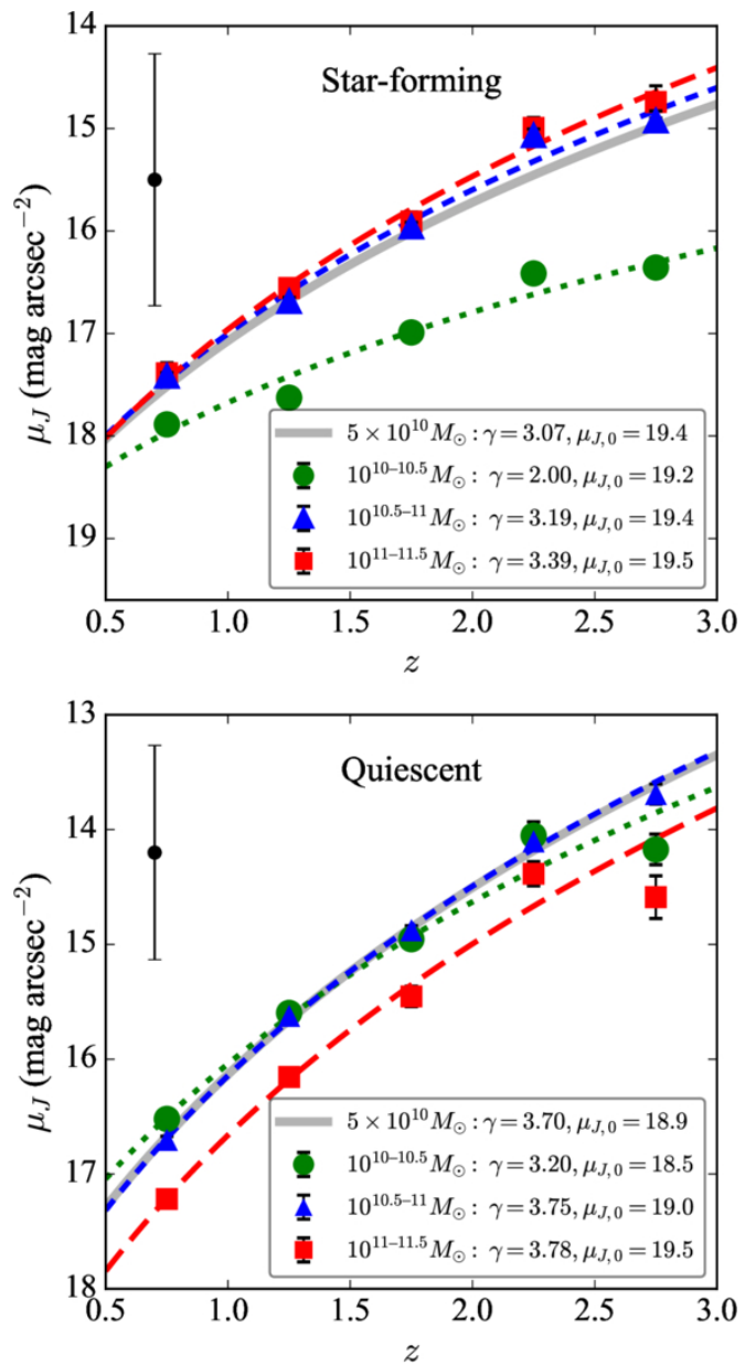
Figure 2. from Si-Yue Yu et al 2026 Astrophys. J. Lett. 1005 doi:10.3847/2041-8213/ae77f8 https://dx.doi.org/10.3847/2041-8213/ae77f8 © 2026. The Author(s). Published by the American Astronomical Society.
