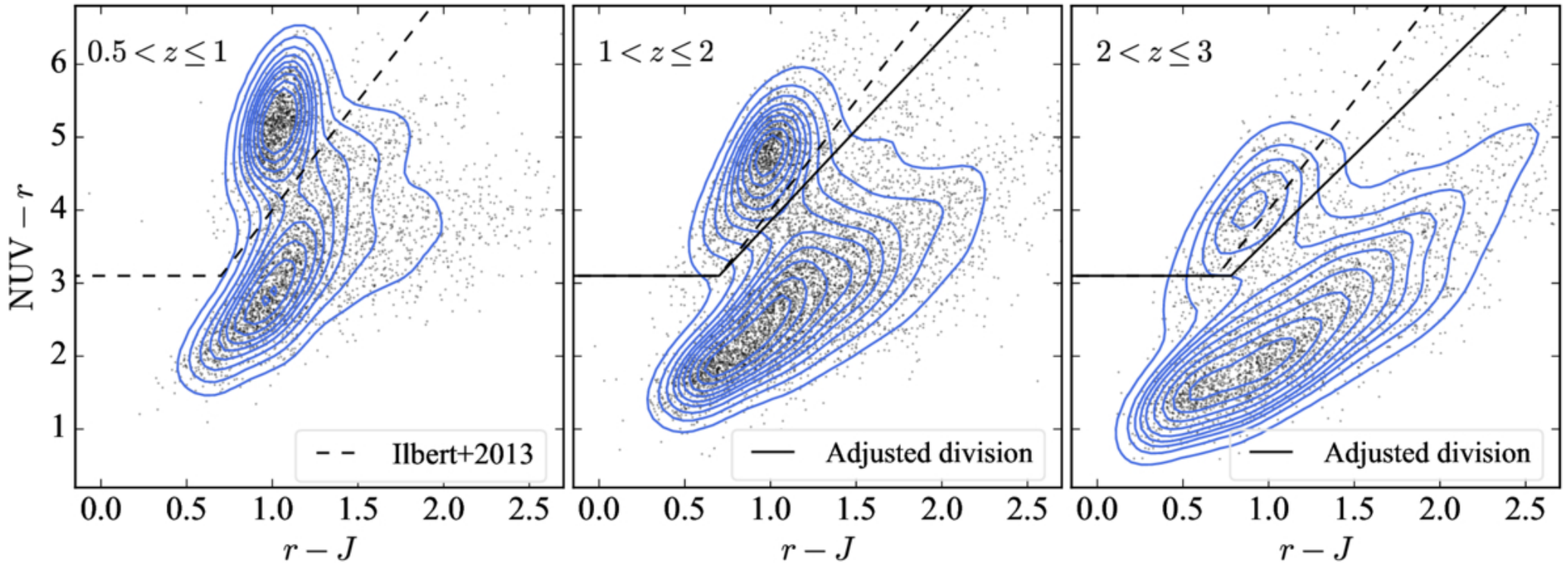
Figure 1. from Si-Yue Yu et al 2026 Astrophys. J. Lett. 1005 doi:10.3847/2041-8213/ae77f8 https://dx.doi.org/10.3847/2041-8213/ae77f8 © 2026. The Author(s). Published by the American Astronomical Society.
