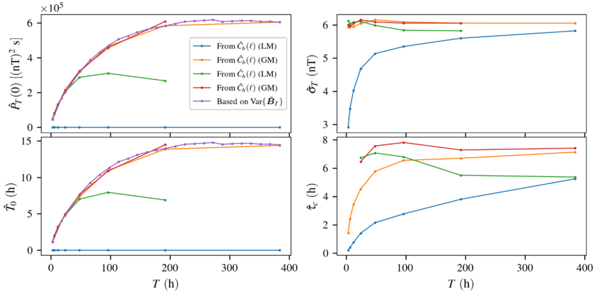
Figure 5. from Jean C. Perez et al 2026 Astrophys. J. Lett. 1005 doi:10.3847/2041-8213/ae77f4 https://dx.doi.org/10.3847/2041-8213/ae77f4 © 2026. The Author(s). Published by the American Astronomical Society.
