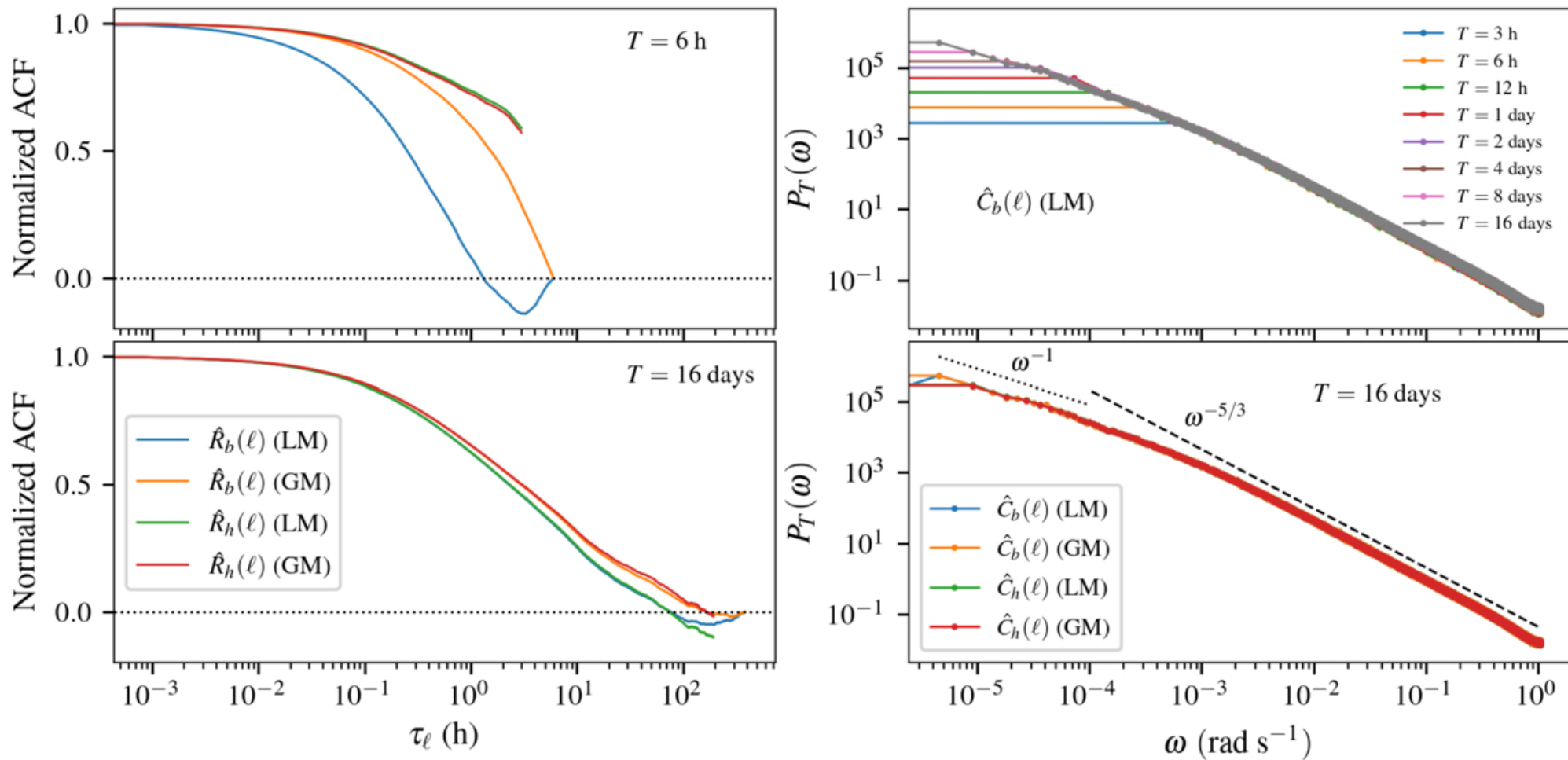
Figure 4. from Jean C. Perez et al 2026 Astrophys. J. Lett. 1005 doi:10.3847/2041-8213/ae77f4 https://dx.doi.org/10.3847/2041-8213/ae77f4 © 2026. The Author(s). Published by the American Astronomical Society.
