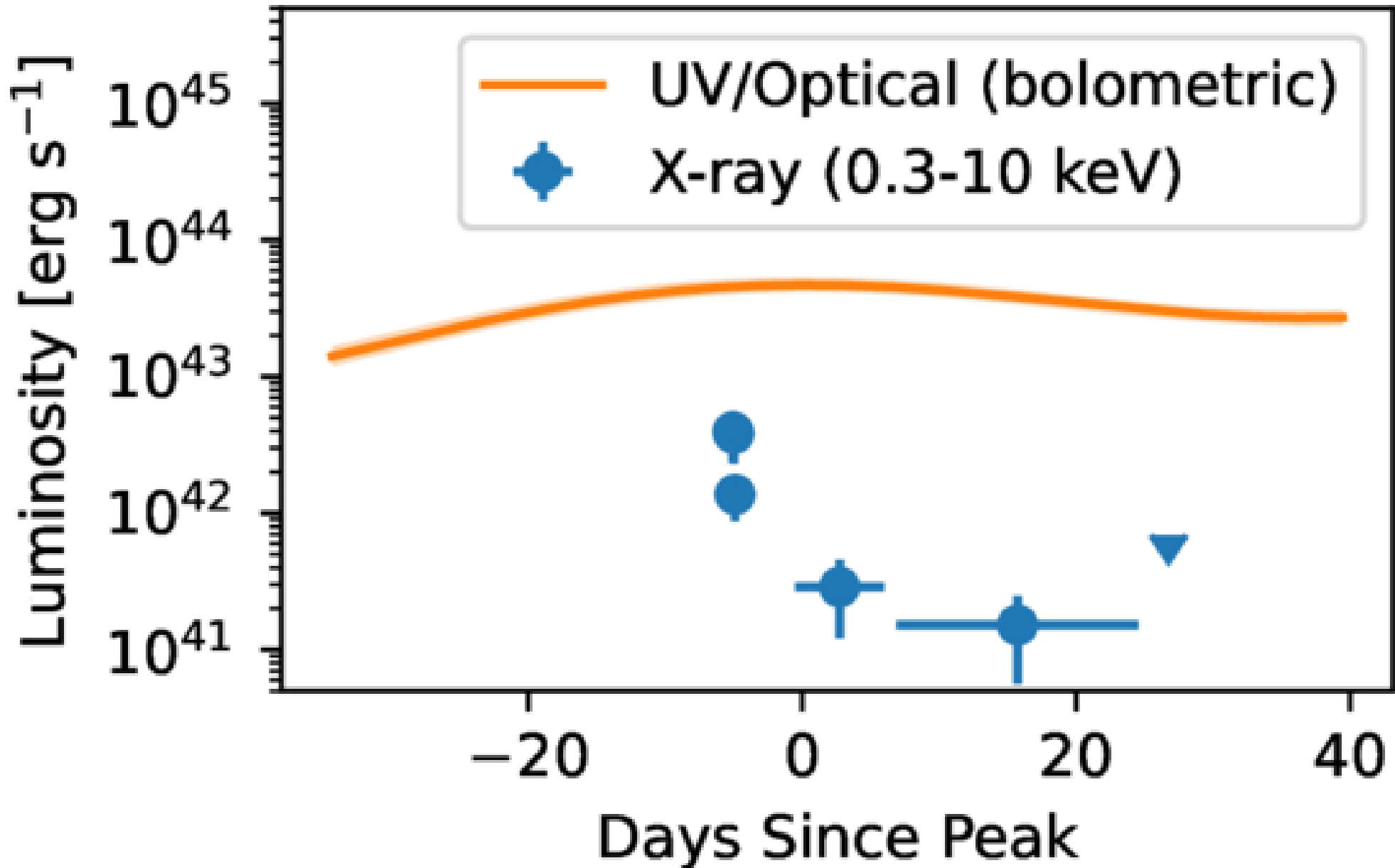
Figure 9. from Robert Stein et al 2026 Astrophys. J. Lett. 1006 doi:10.3847/2041-8213/ae77f3 https://dx.doi.org/10.3847/2041-8213/ae77f3 © 2026. The Author(s). Published by the American Astronomical Society.
