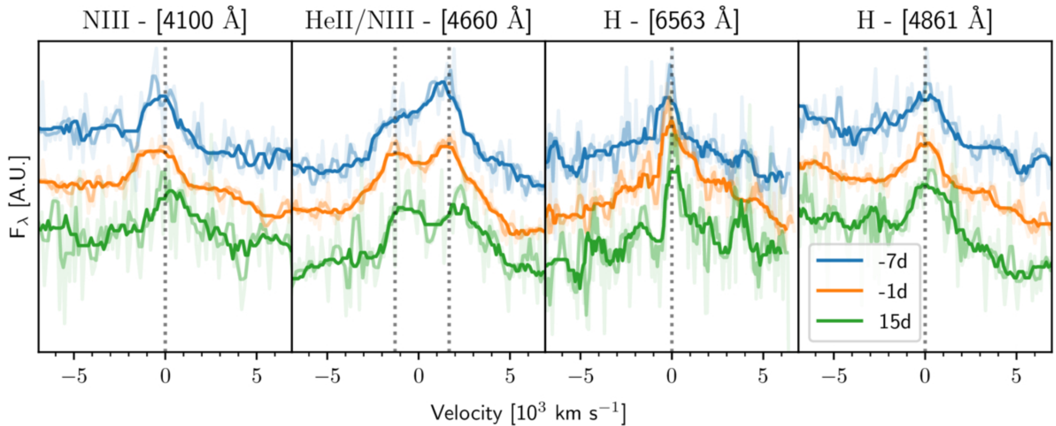
Figure 7. from Robert Stein et al 2026 Astrophys. J. Lett. 1006 doi:10.3847/2041-8213/ae77f3 https://dx.doi.org/10.3847/2041-8213/ae77f3 © 2026. The Author(s). Published by the American Astronomical Society.
