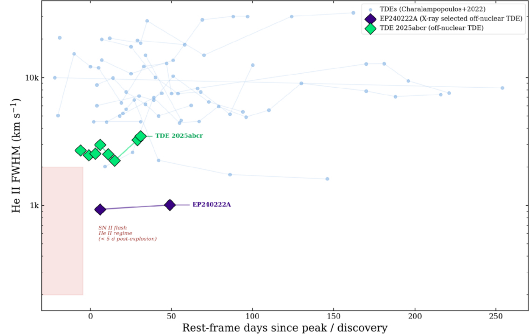
Figure 14. from Robert Stein et al 2026 Astrophys. J. Lett. 1006 doi:10.3847/2041-8213/ae77f3 https://dx.doi.org/10.3847/2041-8213/ae77f3 © 2026. The Author(s). Published by the American Astronomical Society.
