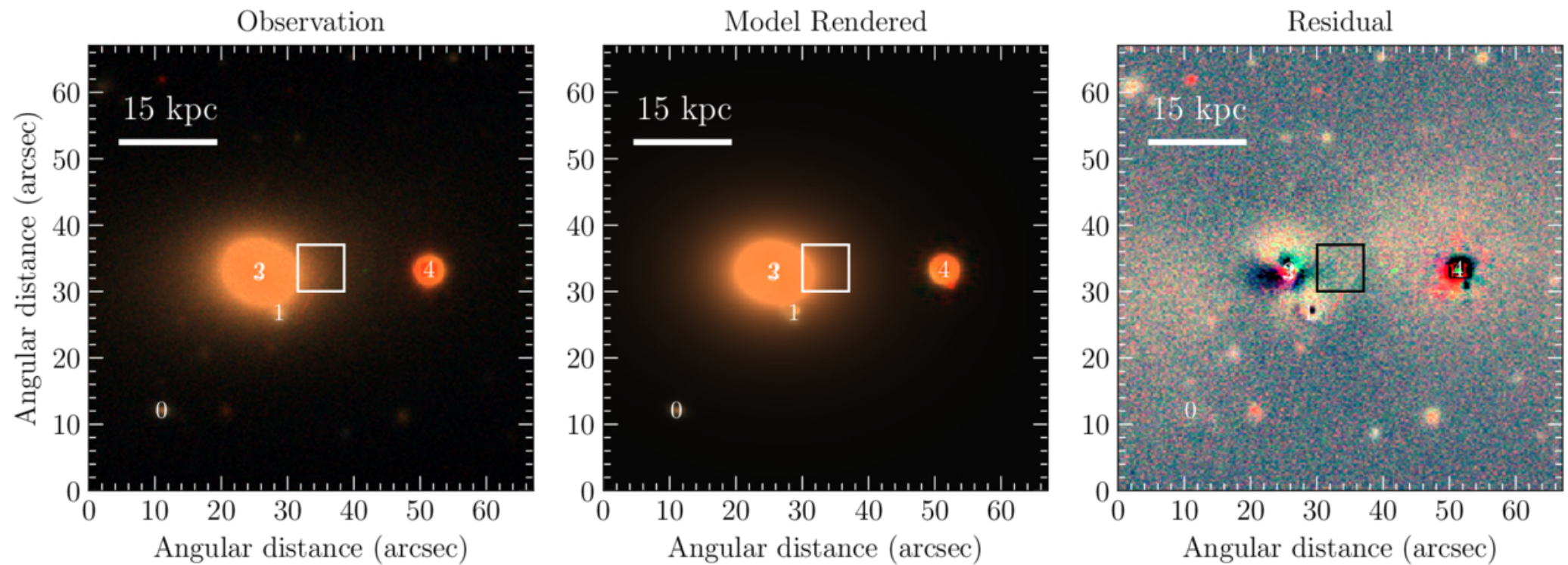
Figure 12. from Robert Stein et al 2026 Astrophys. J. Lett. 1006 doi:10.3847/2041-8213/ae77f3 https://dx.doi.org/10.3847/2041-8213/ae77f3 © 2026. The Author(s). Published by the American Astronomical Society.
