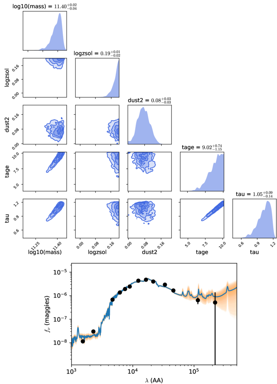
Figure 11. from Robert Stein et al 2026 Astrophys. J. Lett. 1006 doi:10.3847/2041-8213/ae77f3 https://dx.doi.org/10.3847/2041-8213/ae77f3 © 2026. The Author(s). Published by the American Astronomical Society.
