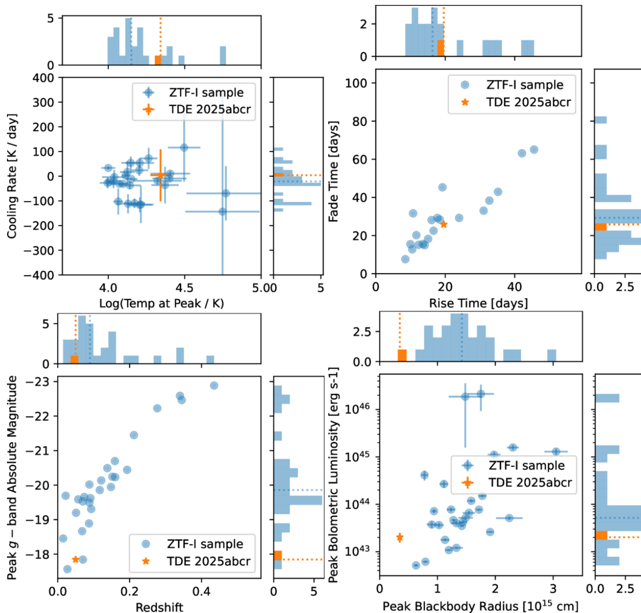
Figure 10. from Robert Stein et al 2026 Astrophys. J. Lett. 1006 doi:10.3847/2041-8213/ae77f3 https://dx.doi.org/10.3847/2041-8213/ae77f3 © 2026. The Author(s). Published by the American Astronomical Society.
