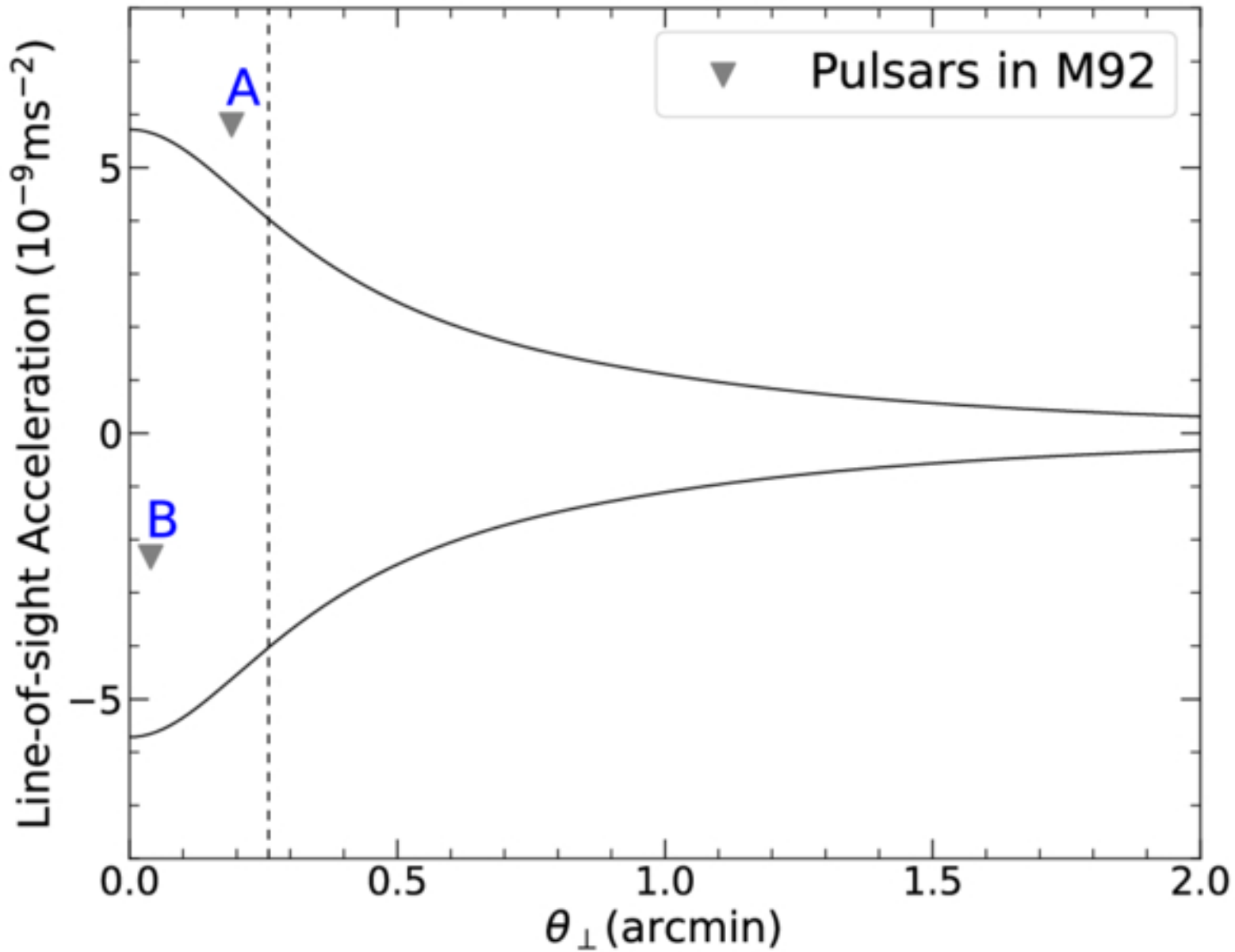
Figure 4. from Dejiang Yin et al 2026 Astrophys. J. Lett. 1004 doi:10.3847/2041-8213/ae77e5 https://dx.doi.org/10.3847/2041-8213/ae77e5 © 2026. The Author(s). Published by the American Astronomical Society.
