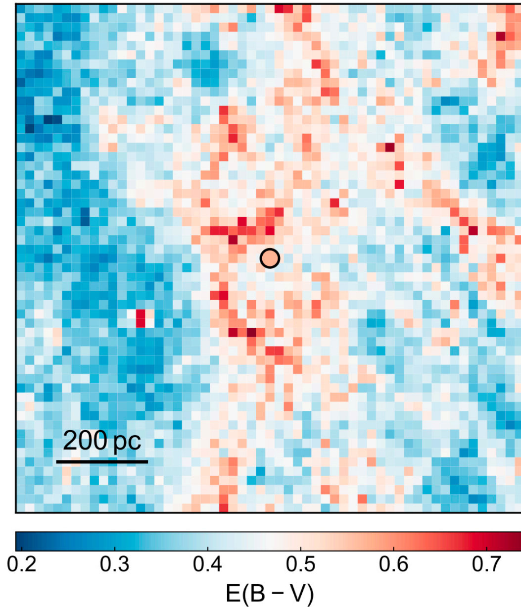
Figure 4. from Pinjian Chen et al 2026 Astrophys. J. Lett. 1005 doi:10.3847/2041-8213/ae77e4 https://dx.doi.org/10.3847/2041-8213/ae77e4 © 2026. The Author(s). Published by the American Astronomical Society.
