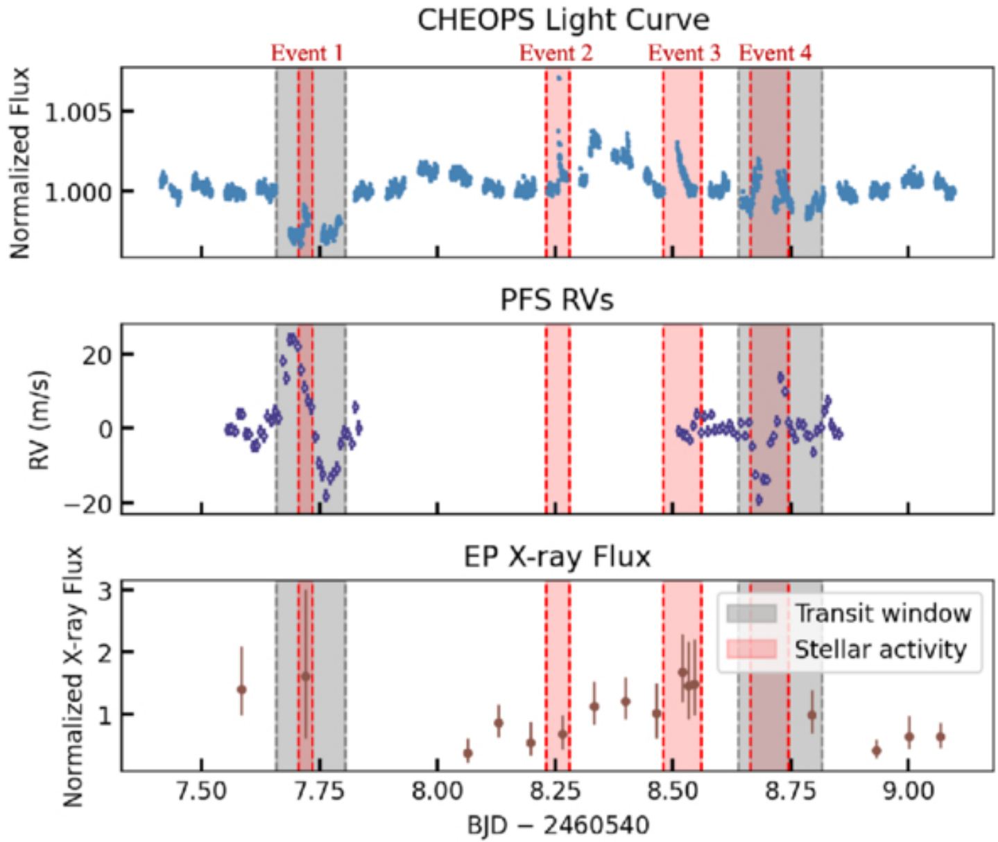
Figure 7. from Zitao Lin et al 2026 Astrophys. J. Lett. 1005 doi:10.3847/2041-8213/ae7725 https://dx.doi.org/10.3847/2041-8213/ae7725 © 2026. The Author(s). Published by the American Astronomical Society.
