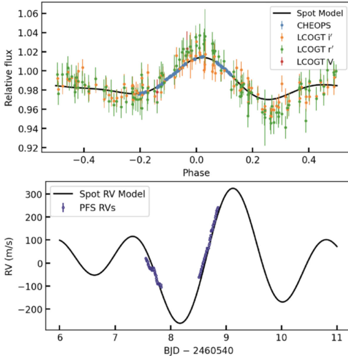
Figure 6. from Zitao Lin et al 2026 Astrophys. J. Lett. 1005 doi:10.3847/2041-8213/ae7725 https://dx.doi.org/10.3847/2041-8213/ae7725 © 2026. The Author(s). Published by the American Astronomical Society.
