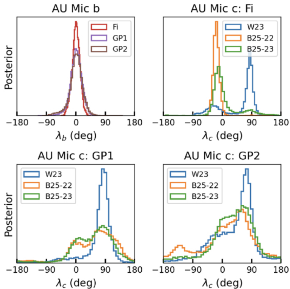
Figure 4. from Zitao Lin et al 2026 Astrophys. J. Lett. 1005 doi:10.3847/2041-8213/ae7725 https://dx.doi.org/10.3847/2041-8213/ae7725 © 2026. The Author(s). Published by the American Astronomical Society.
