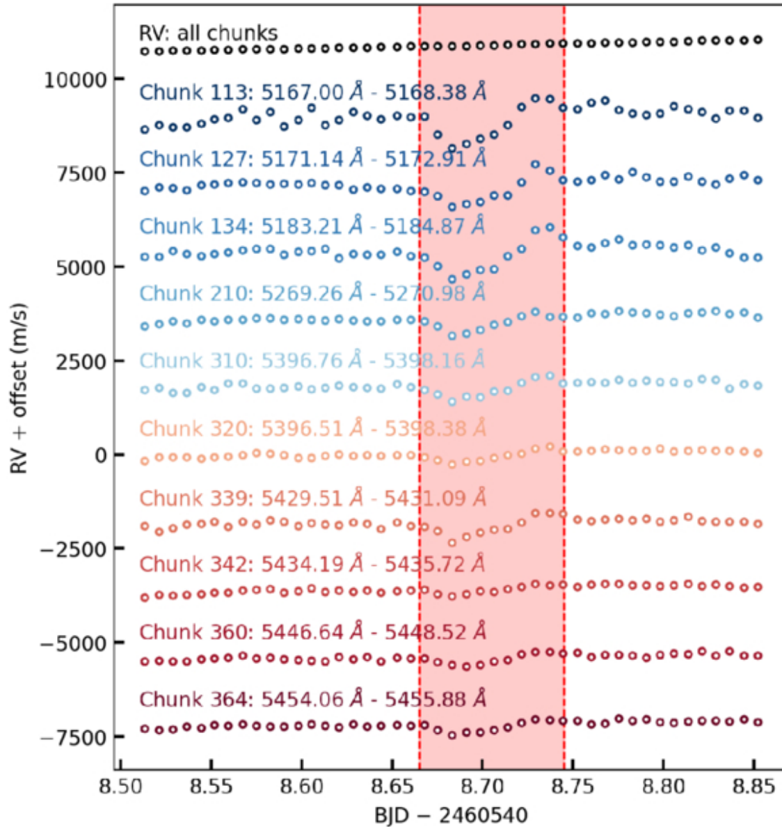
Figure 2. from Zitao Lin et al 2026 Astrophys. J. Lett. 1005 doi:10.3847/2041-8213/ae7725 https://dx.doi.org/10.3847/2041-8213/ae7725 © 2026. The Author(s). Published by the American Astronomical Society.
