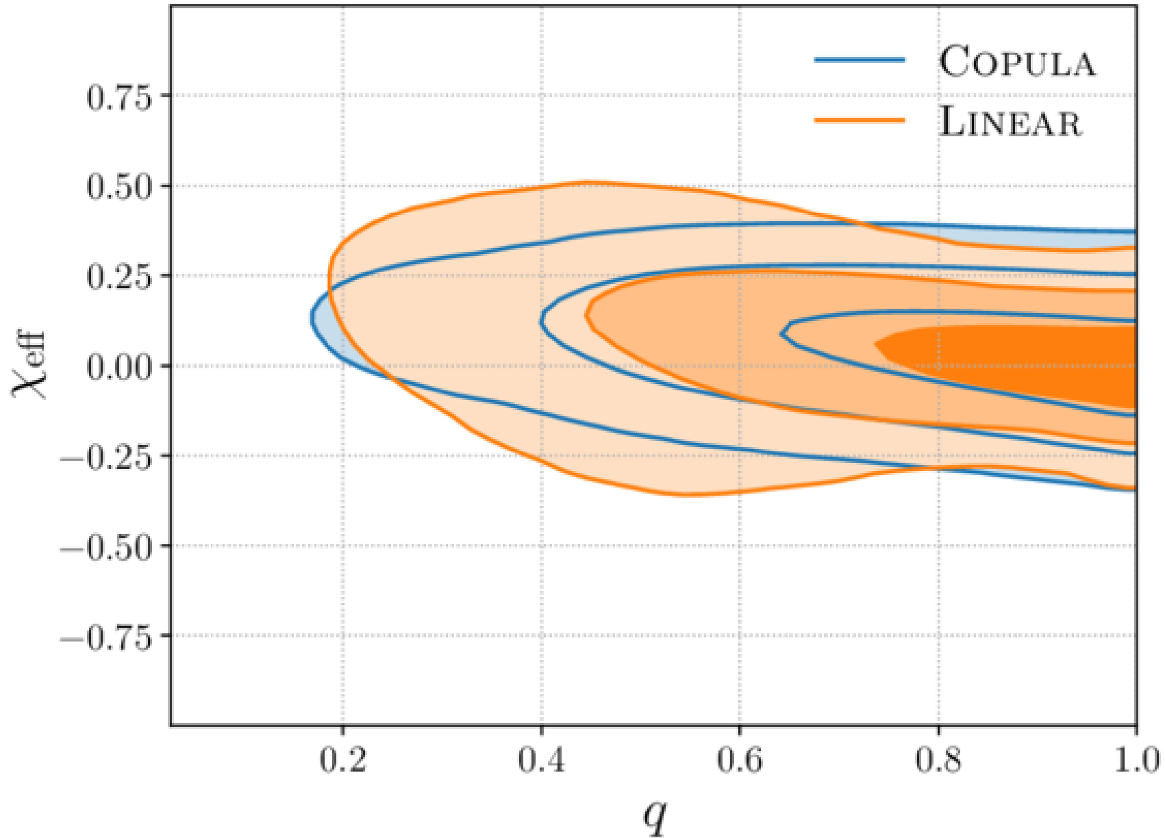
Figure 12. from A. G. Abac et al 2026 Astrophys. J. Lett. 1005 doi:10.3847/2041-8213/ae771e https://dx.doi.org/10.3847/2041-8213/ae771e © 2026. The Author(s). Published by the American Astronomical Society.
