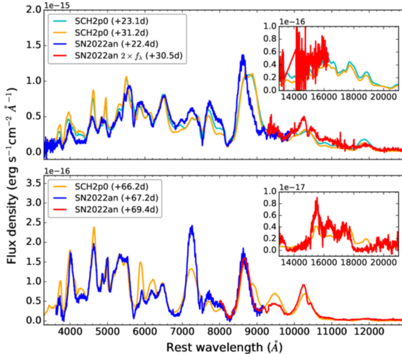
Figure 8. from Ping Chen et al 2026 Astrophys. J. Lett. 1004 doi:10.3847/2041-8213/ae76cf https://dx.doi.org/10.3847/2041-8213/ae76cf © 2026. The Author(s). Published by the American Astronomical Society.
