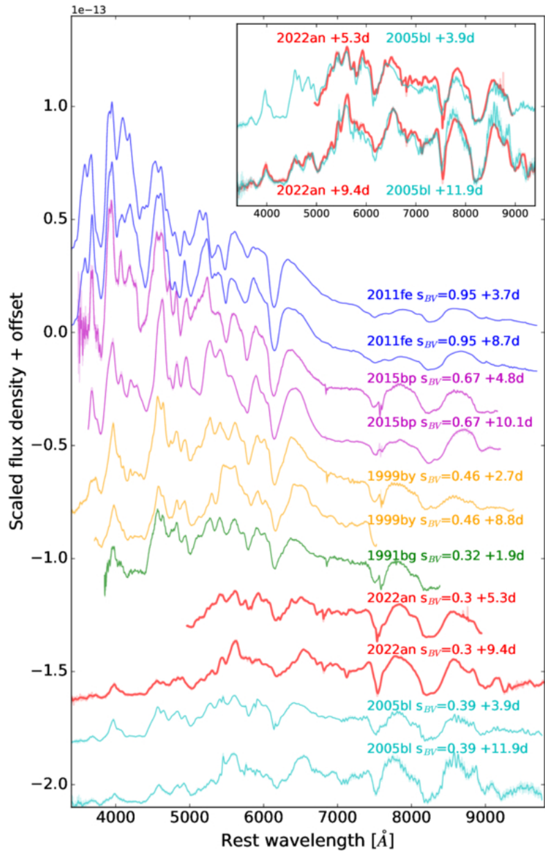
Figure 6. from Ping Chen et al 2026 Astrophys. J. Lett. 1004 doi:10.3847/2041-8213/ae76cf https://dx.doi.org/10.3847/2041-8213/ae76cf © 2026. The Author(s). Published by the American Astronomical Society.
