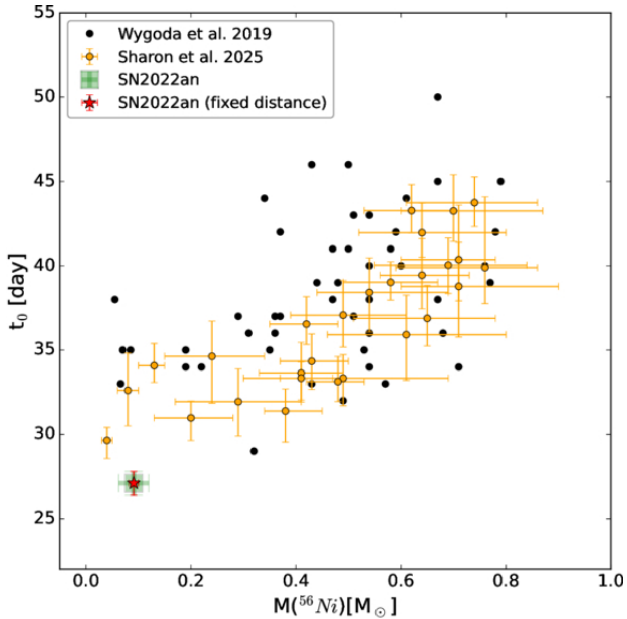
Figure 5. from Ping Chen et al 2026 Astrophys. J. Lett. 1004 doi:10.3847/2041-8213/ae76cf https://dx.doi.org/10.3847/2041-8213/ae76cf © 2026. The Author(s). Published by the American Astronomical Society.
