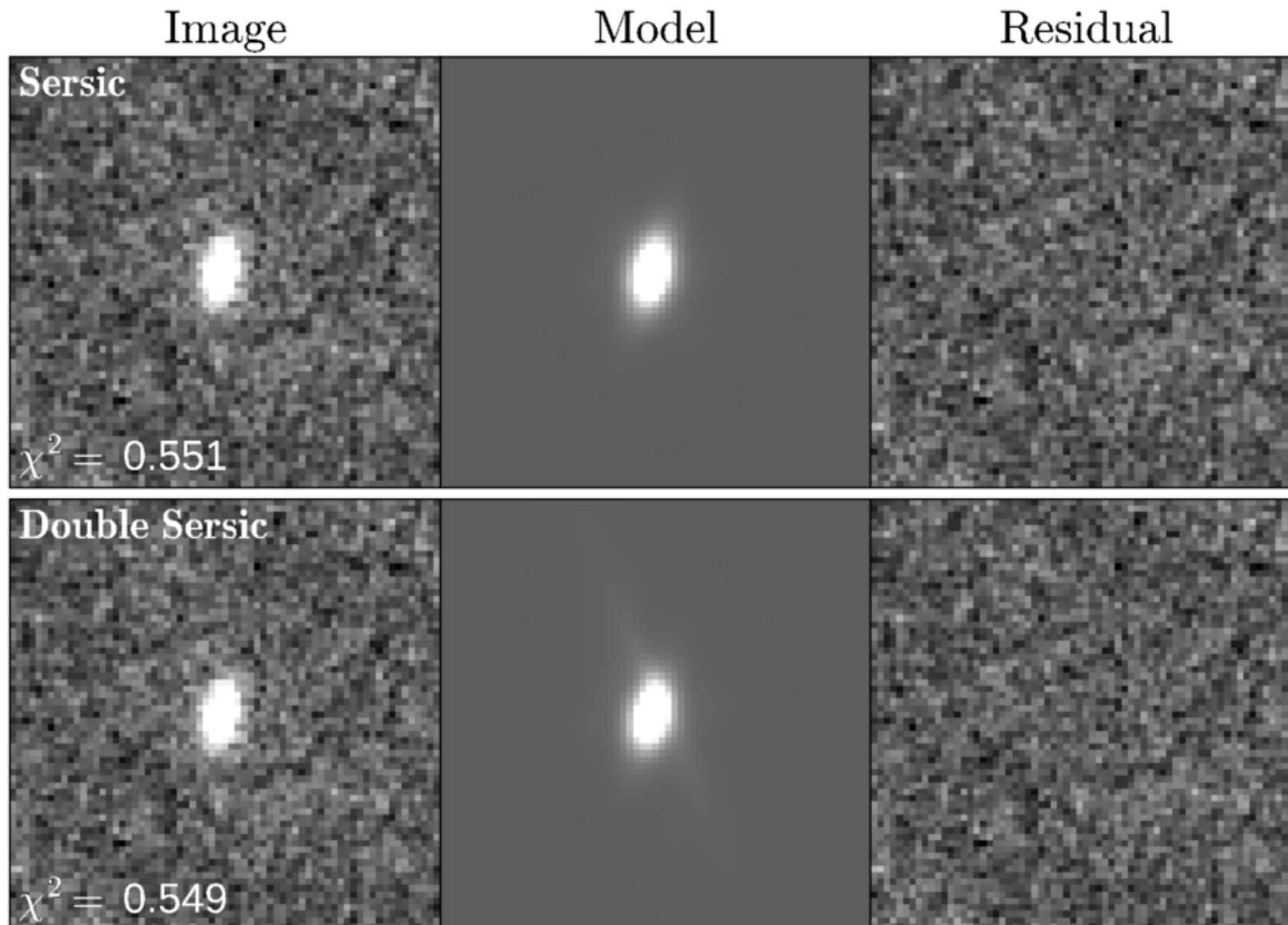
Figure 3. from Shuairu Zhu et al 2026 Astrophys. J. Lett. 1005 doi:10.3847/2041-8213/ae75e1 https://dx.doi.org/10.3847/2041-8213/ae75e1 © 2026. The Author(s). Published by the American Astronomical Society.
