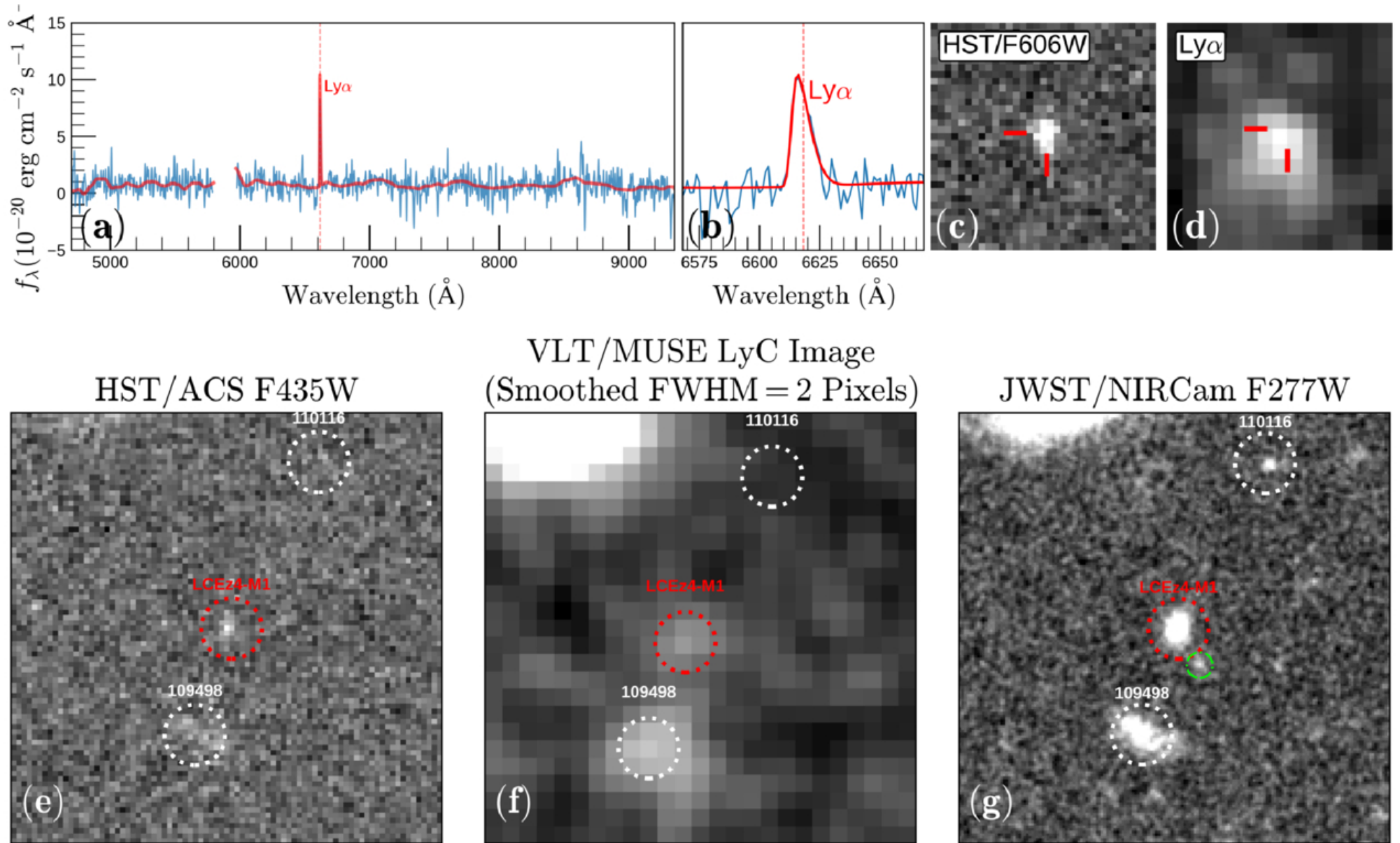
Figure 1. from Shuairu Zhu et al 2026 Astrophys. J. Lett. 1005 doi:10.3847/2041-8213/ae75e1 https://dx.doi.org/10.3847/2041-8213/ae75e1 © 2026. The Author(s). Published by the American Astronomical Society.
