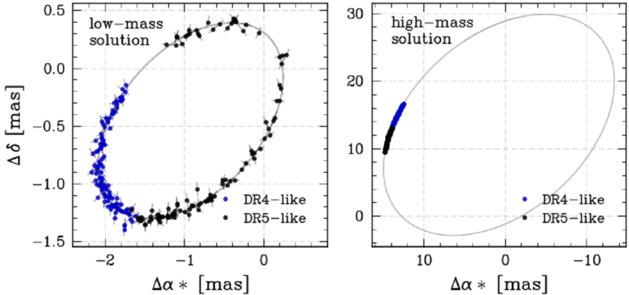
Figure 6. from Eritas Yang et al 2026 Astrophys. J. Lett. 1004 doi:10.3847/2041-8213/ae7570 https://dx.doi.org/10.3847/2041-8213/ae7570 © 2026. The Author(s). Published by the American Astronomical Society.
