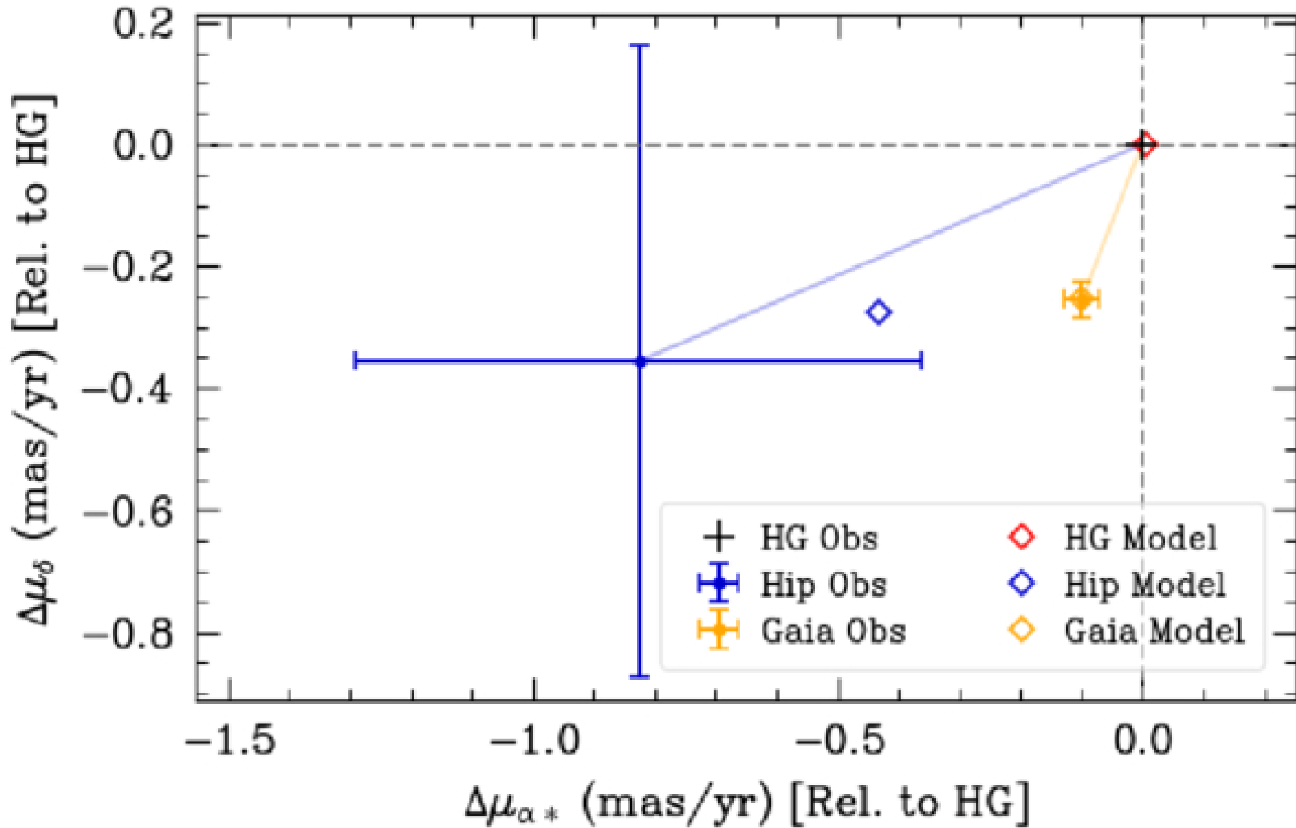
Figure 4. from Eritas Yang et al 2026 Astrophys. J. Lett. 1004 doi:10.3847/2041-8213/ae7570 https://dx.doi.org/10.3847/2041-8213/ae7570 © 2026. The Author(s). Published by the American Astronomical Society.
