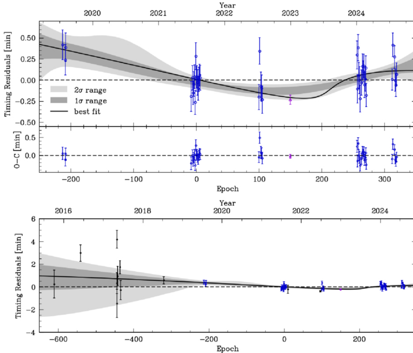
Figure 3. from Eritas Yang et al 2026 Astrophys. J. Lett. 1004 doi:10.3847/2041-8213/ae7570 https://dx.doi.org/10.3847/2041-8213/ae7570 © 2026. The Author(s). Published by the American Astronomical Society.
