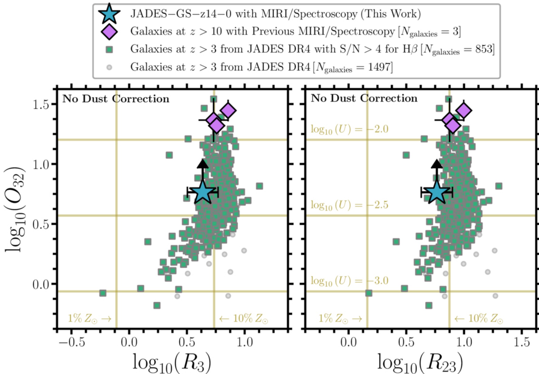
Figure 6. from Jakob M. Helton et al 2026 Astrophys. J. Lett. 1004 doi:10.3847/2041-8213/ae7446 https://dx.doi.org/10.3847/2041-8213/ae7446 © 2026. The Author(s). Published by the American Astronomical Society.
