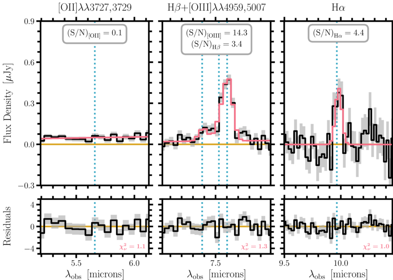
Figure 3. from Jakob M. Helton et al 2026 Astrophys. J. Lett. 1004 doi:10.3847/2041-8213/ae7446 https://dx.doi.org/10.3847/2041-8213/ae7446 © 2026. The Author(s). Published by the American Astronomical Society.
