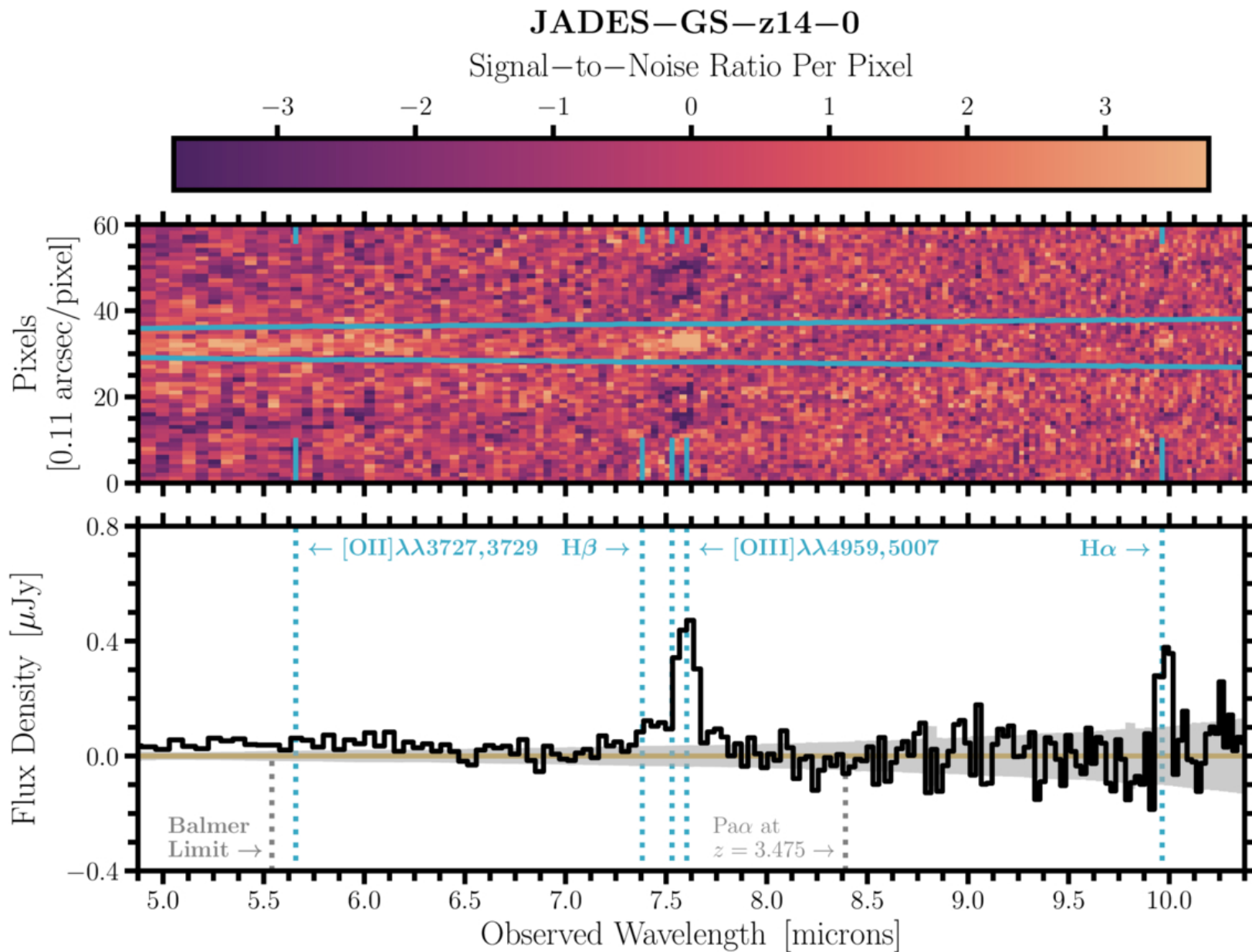
Figure 2. from Jakob M. Helton et al 2026 Astrophys. J. Lett. 1004 doi:10.3847/2041-8213/ae7446 https://dx.doi.org/10.3847/2041-8213/ae7446 © 2026. The Author(s). Published by the American Astronomical Society.
