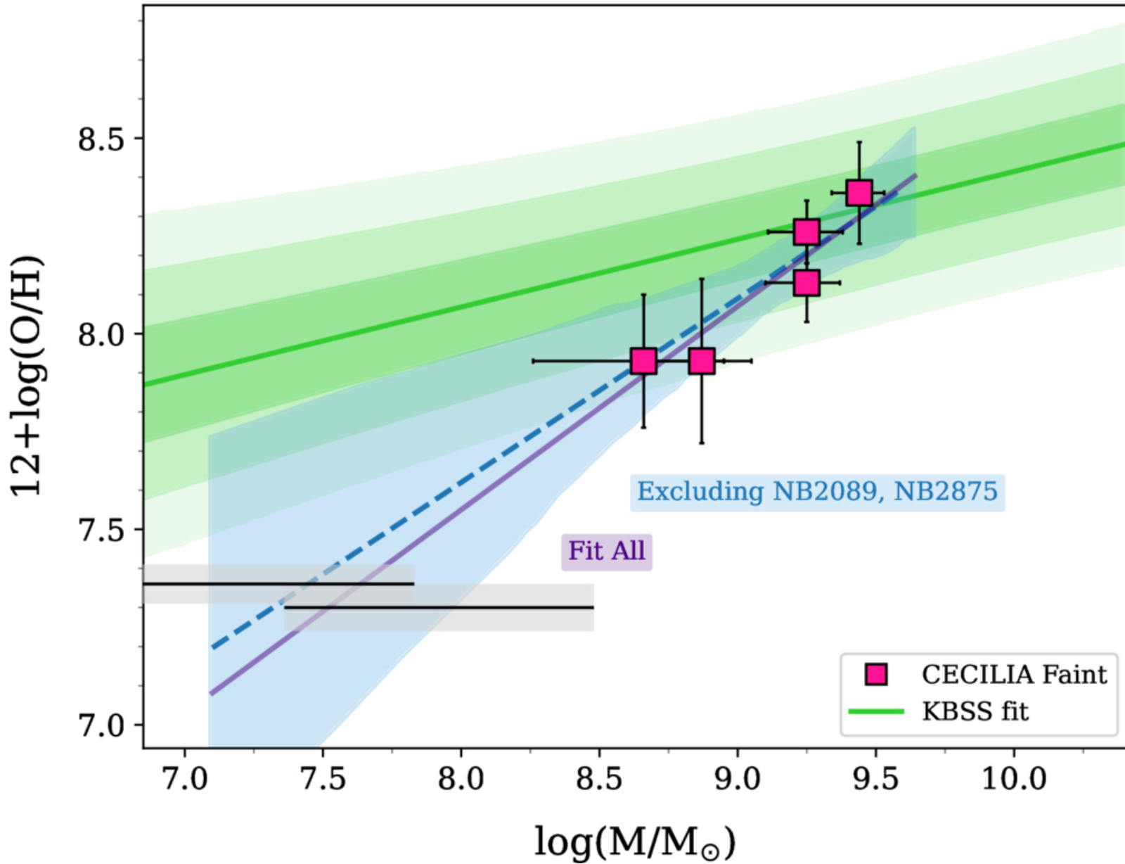
Figure 9. from Menelaos Raptis et al 2026 Astrophys. J. Lett. 1004 doi:10.3847/2041-8213/ae7445 https://dx.doi.org/10.3847/2041-8213/ae7445 © 2026. The Author(s). Published by the American Astronomical Society.
