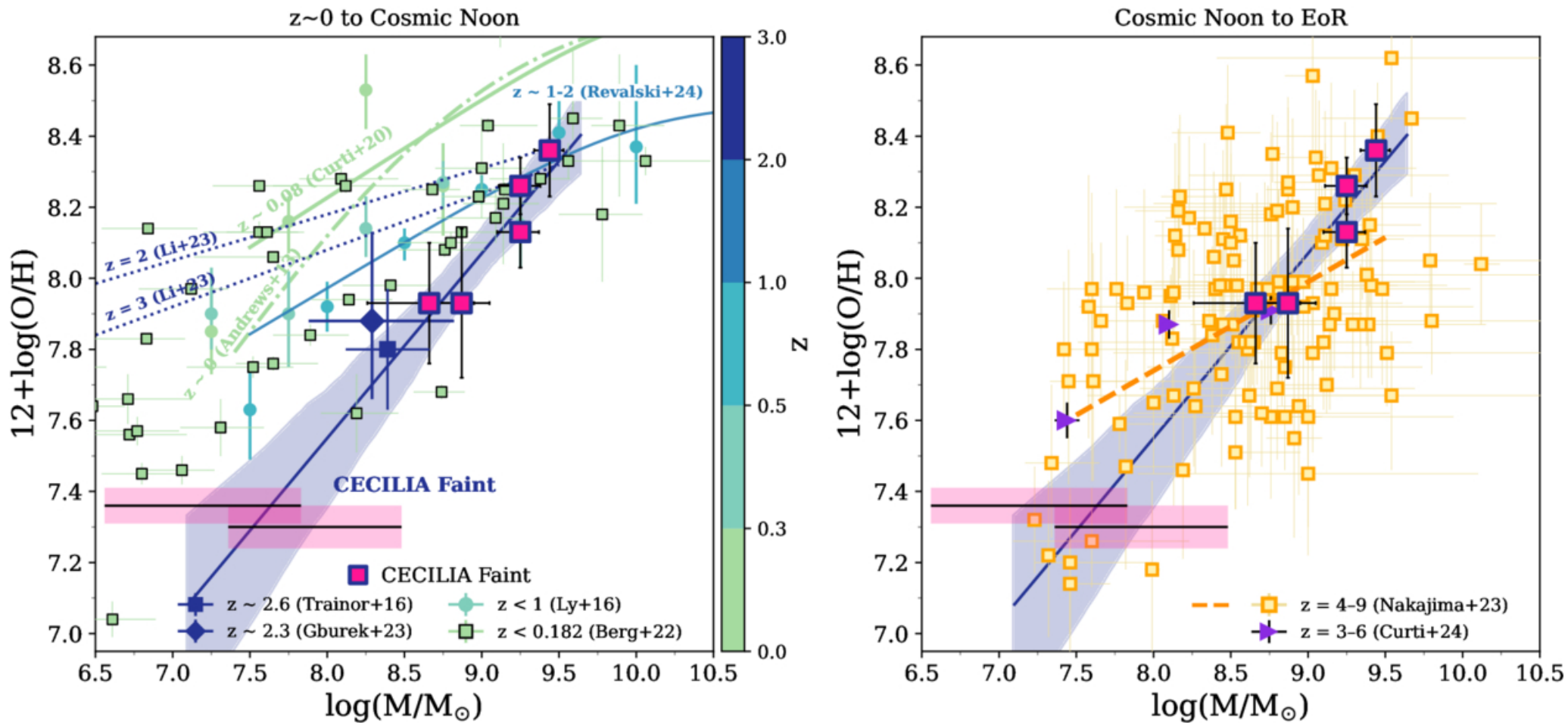
Figure 7. from Menelaos Raptis et al 2026 Astrophys. J. Lett. 1004 doi:10.3847/2041-8213/ae7445 https://dx.doi.org/10.3847/2041-8213/ae7445 © 2026. The Author(s). Published by the American Astronomical Society.
