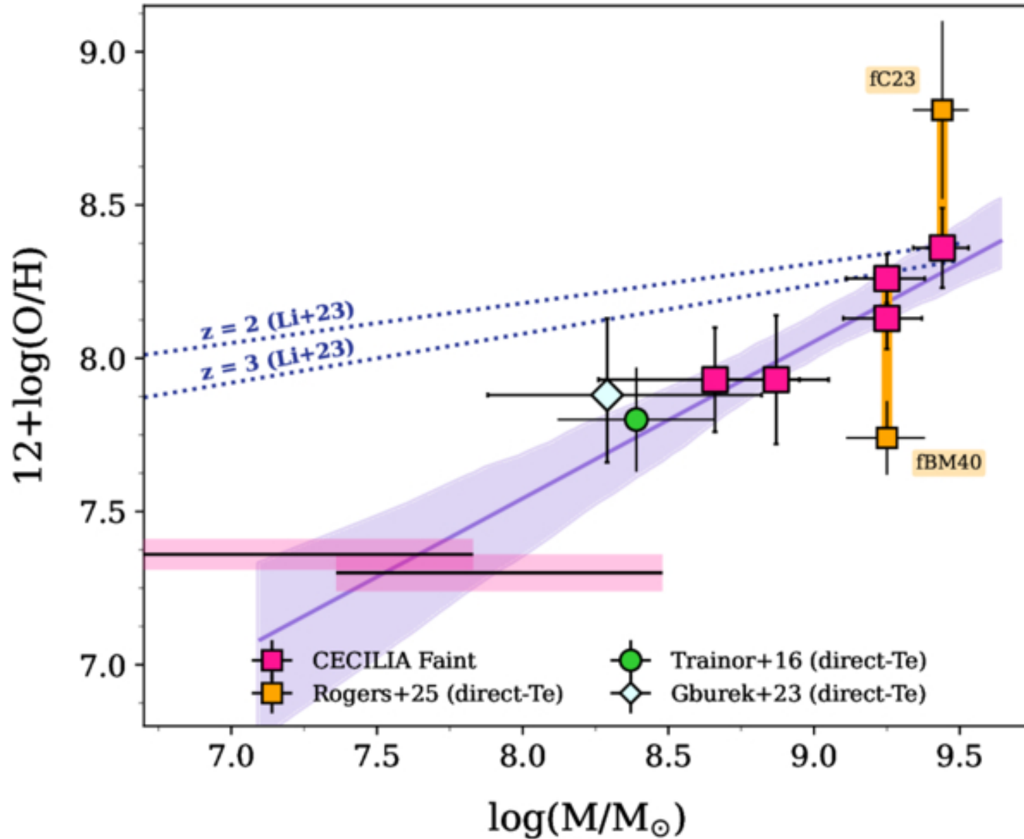
Figure 6. from Menelaos Raptis et al 2026 Astrophys. J. Lett. 1004 doi:10.3847/2041-8213/ae7445 https://dx.doi.org/10.3847/2041-8213/ae7445 © 2026. The Author(s). Published by the American Astronomical Society.
