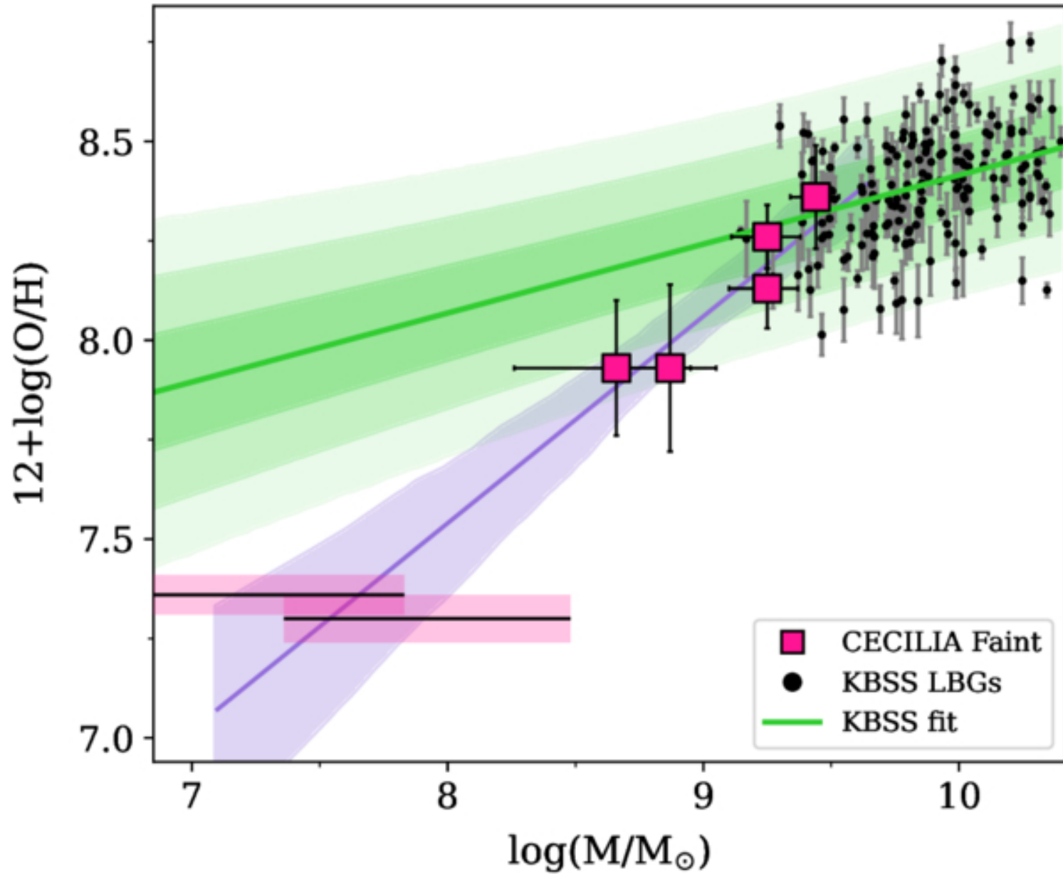
Figure 5. from Menelaos Raptis et al 2026 Astrophys. J. Lett. 1004 doi:10.3847/2041-8213/ae7445 https://dx.doi.org/10.3847/2041-8213/ae7445 © 2026. The Author(s). Published by the American Astronomical Society.
