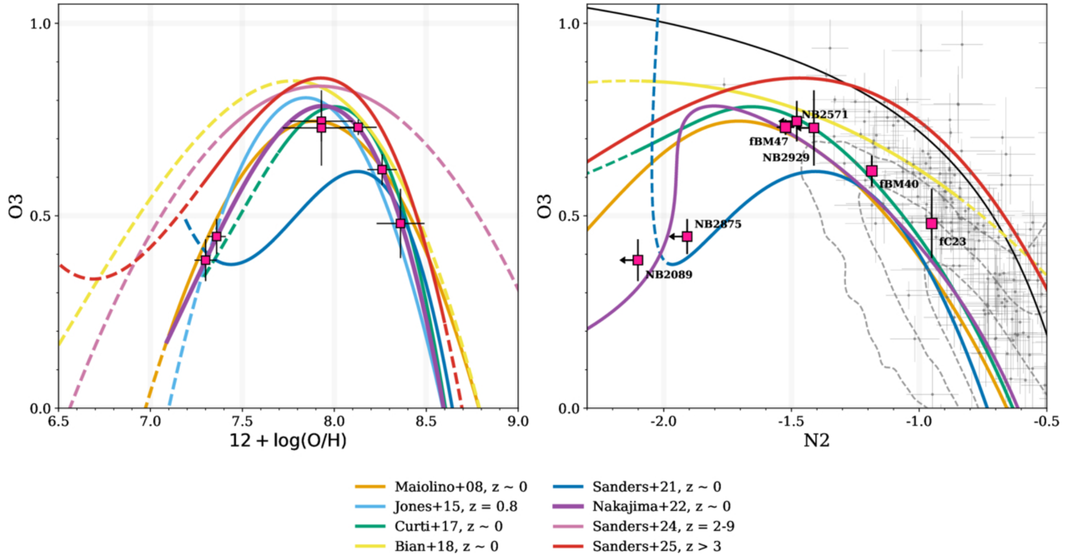
Figure 3. from Menelaos Raptis et al 2026 Astrophys. J. Lett. 1004 doi:10.3847/2041-8213/ae7445 https://dx.doi.org/10.3847/2041-8213/ae7445 © 2026. The Author(s). Published by the American Astronomical Society.
