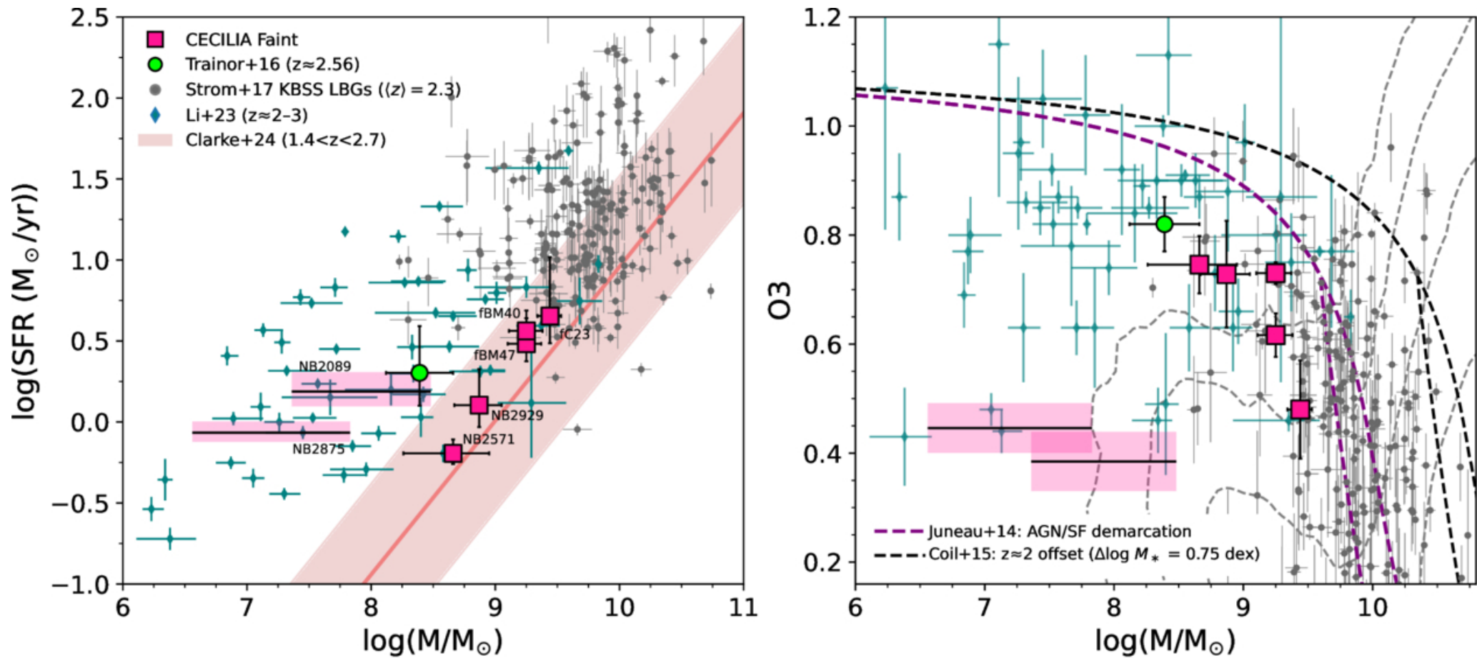
Figure 2. from Menelaos Raptis et al 2026 Astrophys. J. Lett. 1004 doi:10.3847/2041-8213/ae7445 https://dx.doi.org/10.3847/2041-8213/ae7445 © 2026. The Author(s). Published by the American Astronomical Society.
