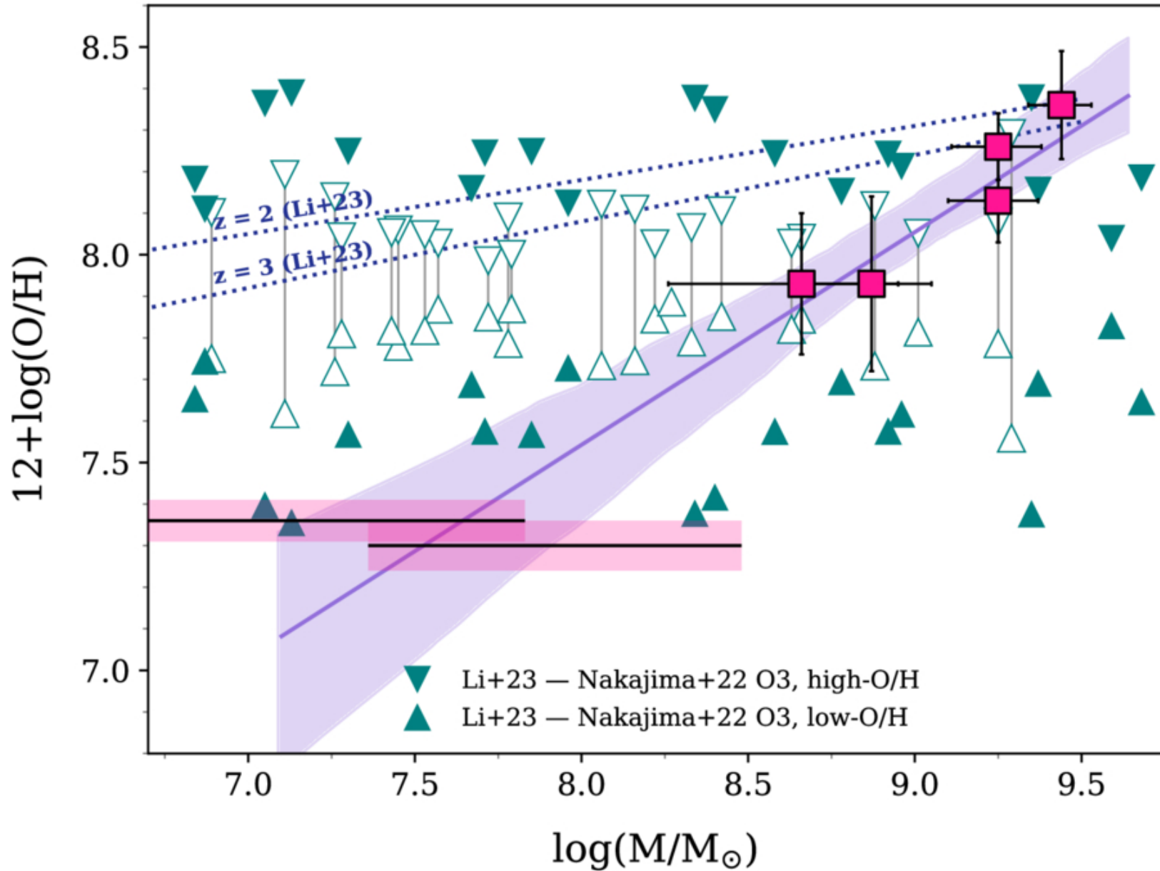
Figure 10. from Menelaos Raptis et al 2026 Astrophys. J. Lett. 1004 doi:10.3847/2041-8213/ae7445 https://dx.doi.org/10.3847/2041-8213/ae7445 © 2026. The Author(s). Published by the American Astronomical Society.
