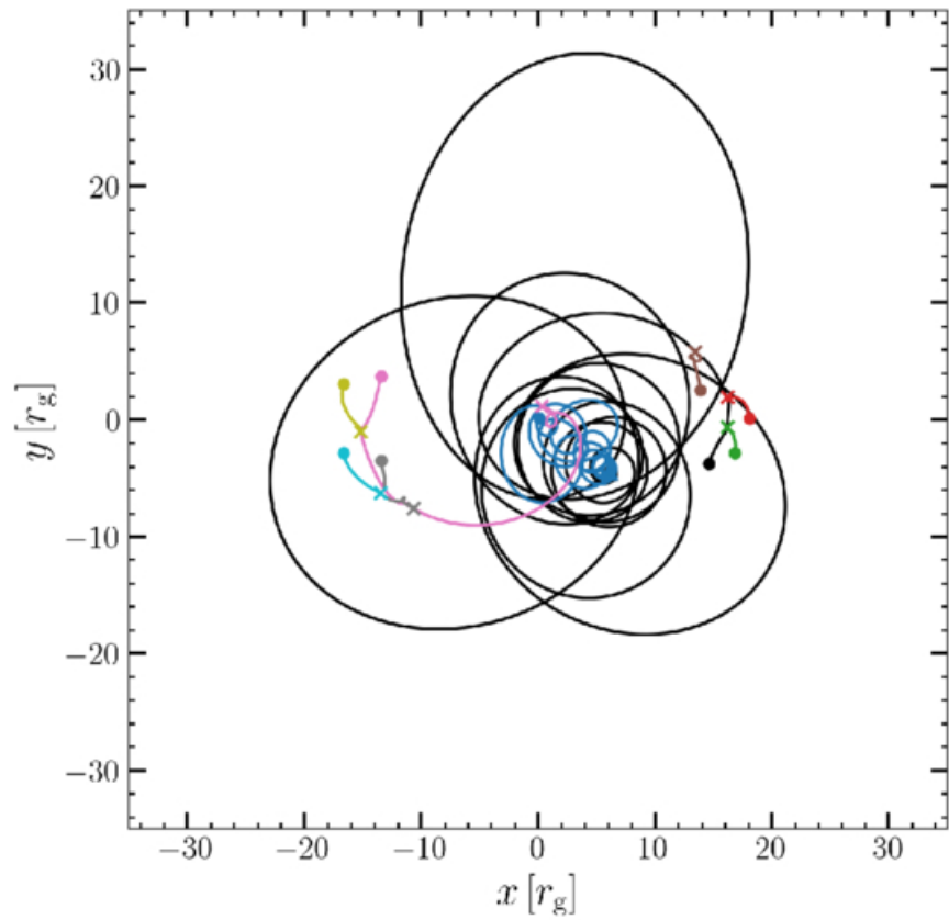
Figure 2. from Jiaxi Wu et al 2026 Astrophys. J. Lett. 1004 doi:10.3847/2041-8213/ae743a https://dx.doi.org/10.3847/2041-8213/ae743a © 2026. The Author(s). Published by the American Astronomical Society.
