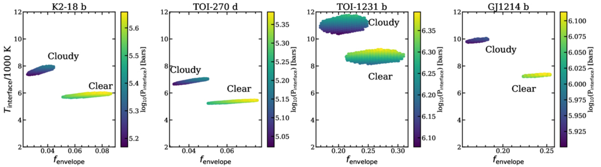
Figure 6. from Sagnick Mukherjee et al 2026 Astrophys. J. Lett. 1005 doi:10.3847/2041-8213/ae7432 https://dx.doi.org/10.3847/2041-8213/ae7432 © 2026. The Author(s). Published by the American Astronomical Society.
