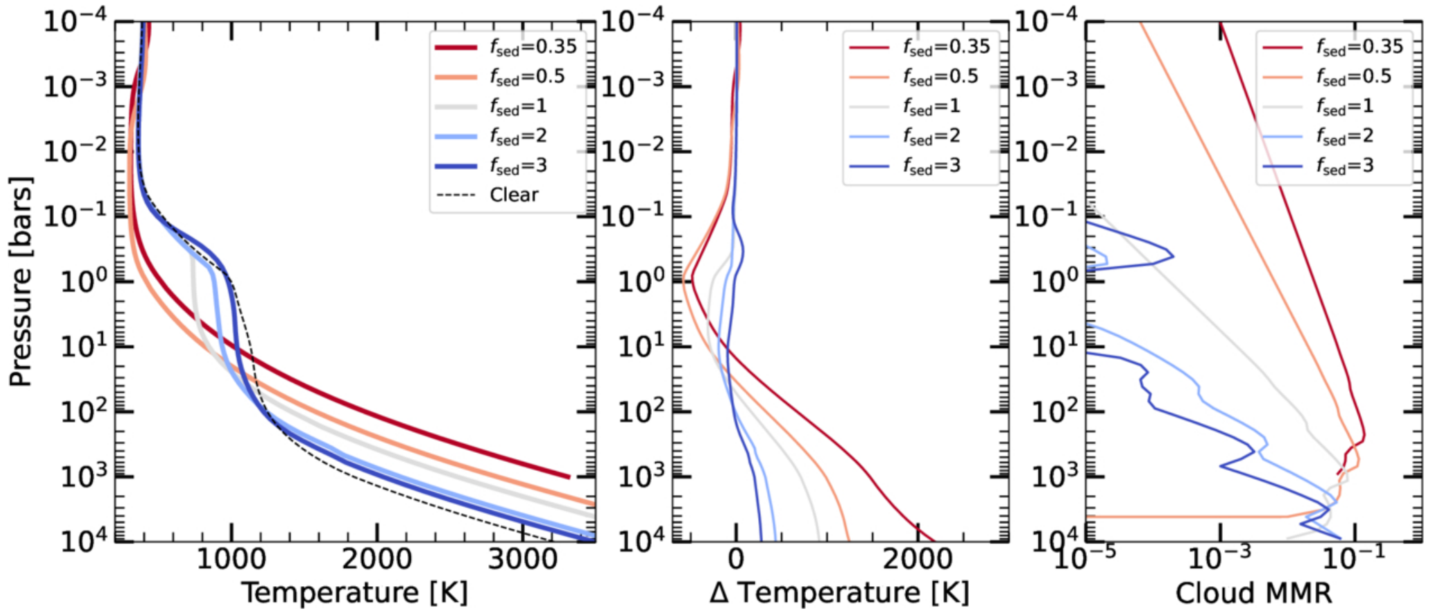
Figure 2. from Sagnick Mukherjee et al 2026 Astrophys. J. Lett. 1005 doi:10.3847/2041-8213/ae7432 https://dx.doi.org/10.3847/2041-8213/ae7432 © 2026. The Author(s). Published by the American Astronomical Society.
