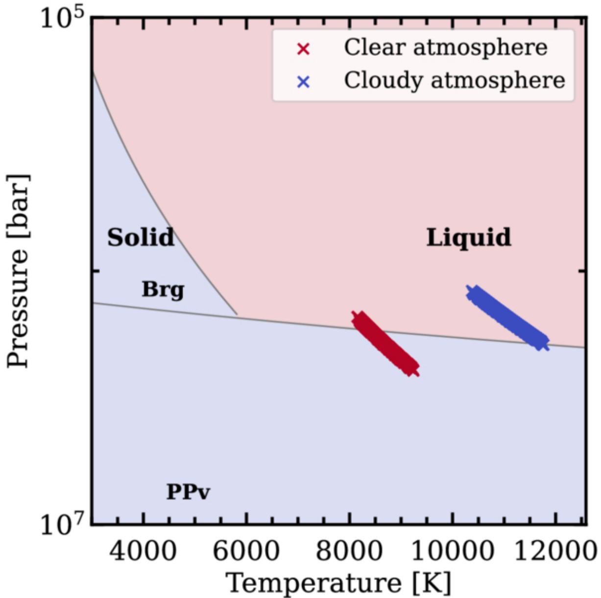
Figure 10. from Sagnick Mukherjee et al 2026 Astrophys. J. Lett. 1005 doi:10.3847/2041-8213/ae7432 https://dx.doi.org/10.3847/2041-8213/ae7432 © 2026. The Author(s). Published by the American Astronomical Society.
