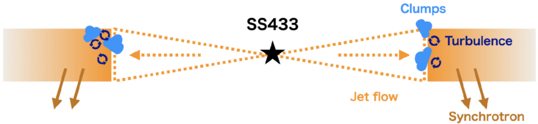
Figure 5. from Haruka Sakemi et al 2026 Astrophys. J. Lett. 1004 doi:10.3847/2041-8213/ae736b https://dx.doi.org/10.3847/2041-8213/ae736b © 2026. The Author(s). Published by the American Astronomical Society.
