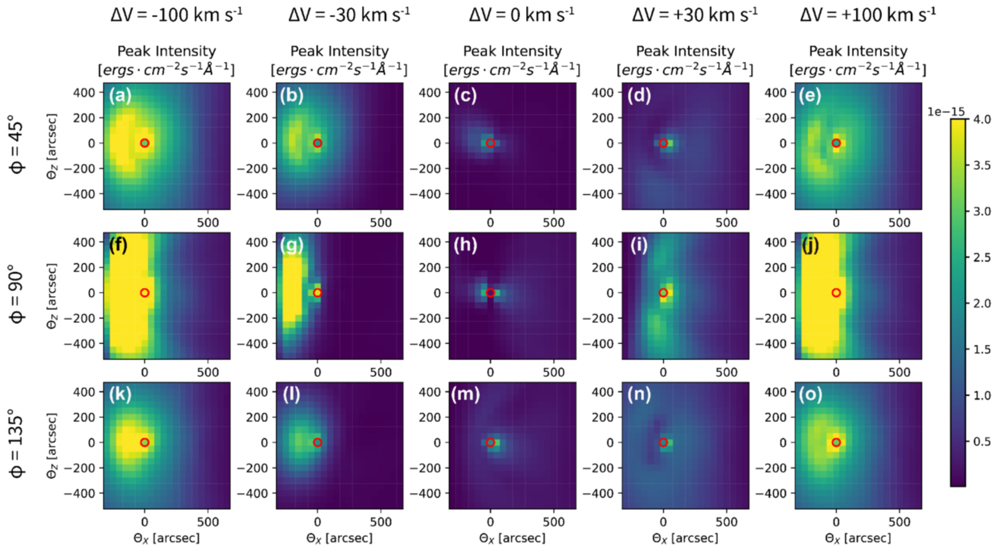
Figure 7. from Ziqi Wu et al 2026 Astrophys. J. Lett. 1005 doi:10.3847/2041-8213/ae7369 https://dx.doi.org/10.3847/2041-8213/ae7369 © 2026. The Author(s). Published by the American Astronomical Society.
