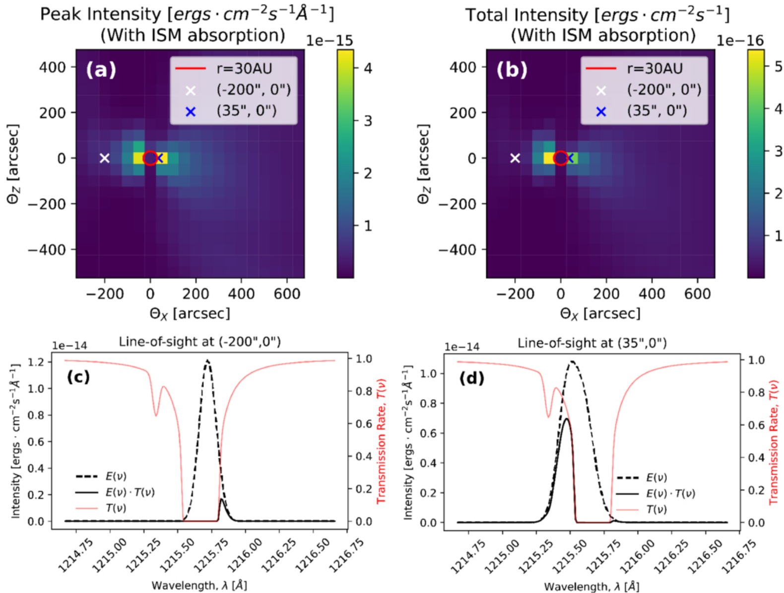
Figure 5. from Ziqi Wu et al 2026 Astrophys. J. Lett. 1005 doi:10.3847/2041-8213/ae7369 https://dx.doi.org/10.3847/2041-8213/ae7369 © 2026. The Author(s). Published by the American Astronomical Society.
