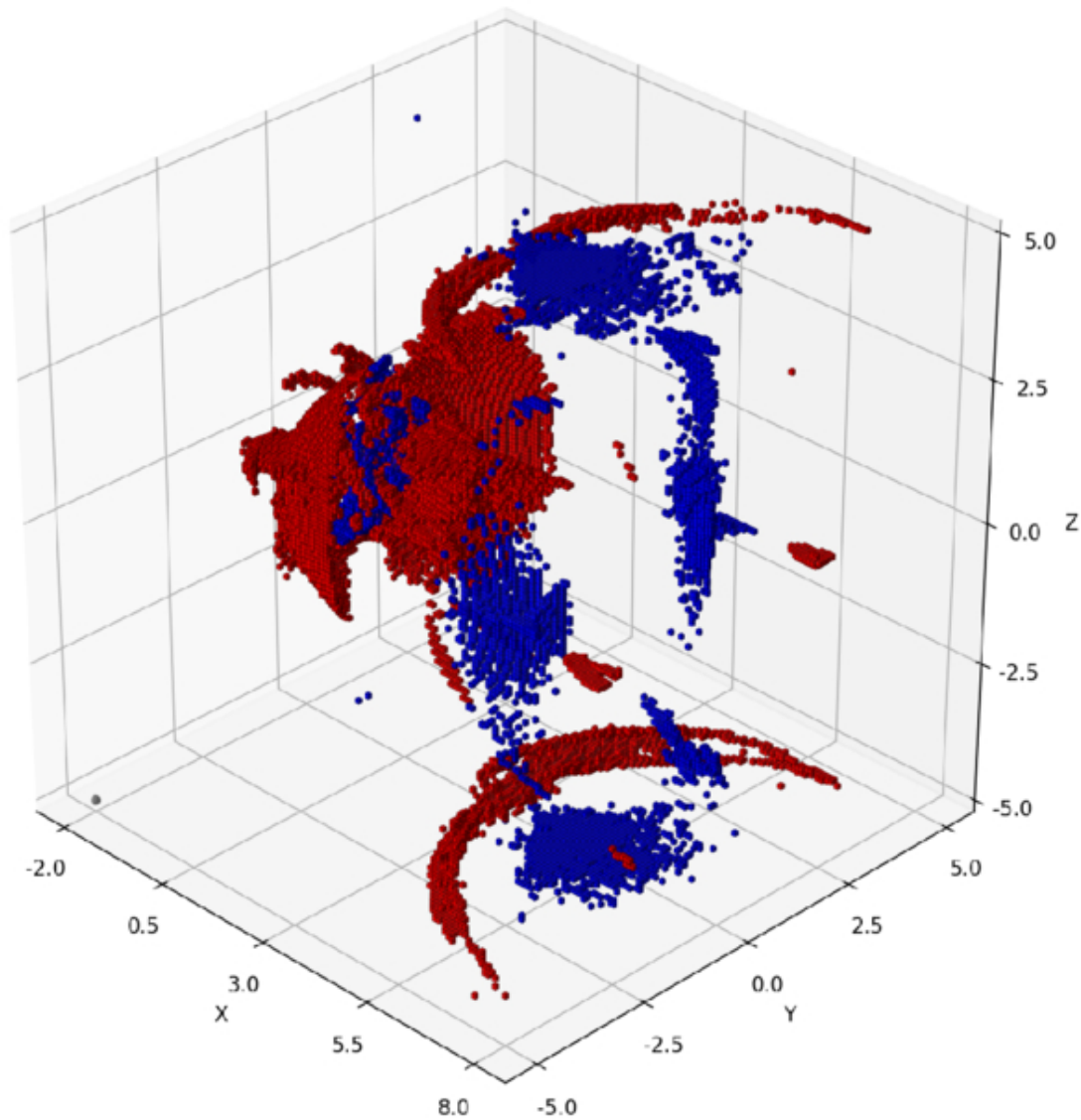
3D Voxel Isosurface of J.E
