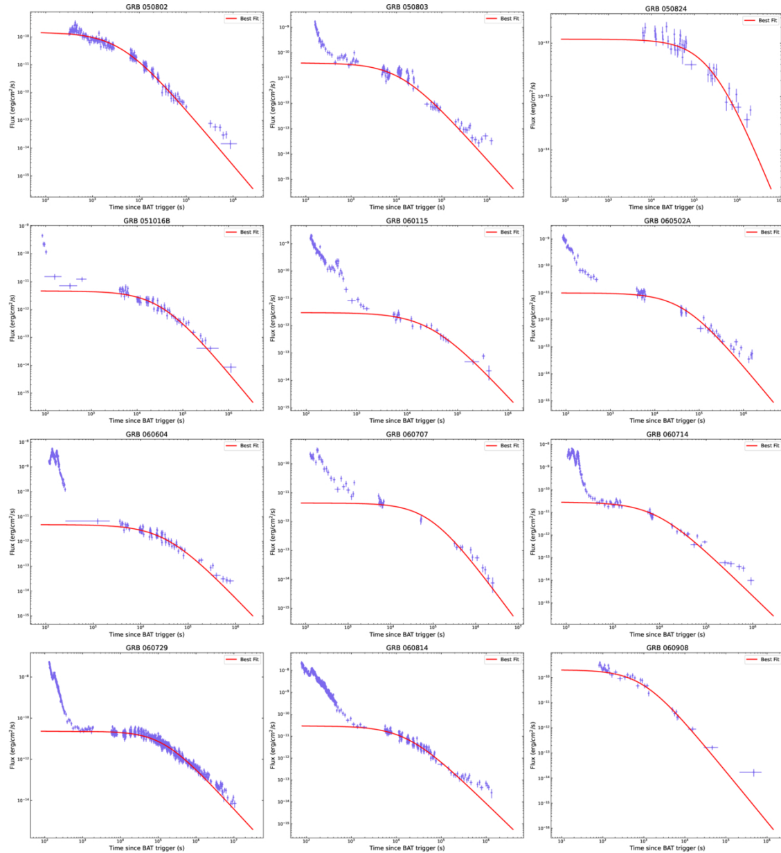
Figure 1. The blue data points are from Swift/XRT observations, while the red line represents the best model to the data. from Yu-Qi Zhou et al 2026 Astrophys. J. Lett. 1004 doi:10.3847/2041-8213/ae7329 https://dx.doi.org/10.3847/2041-8213/ae7329
