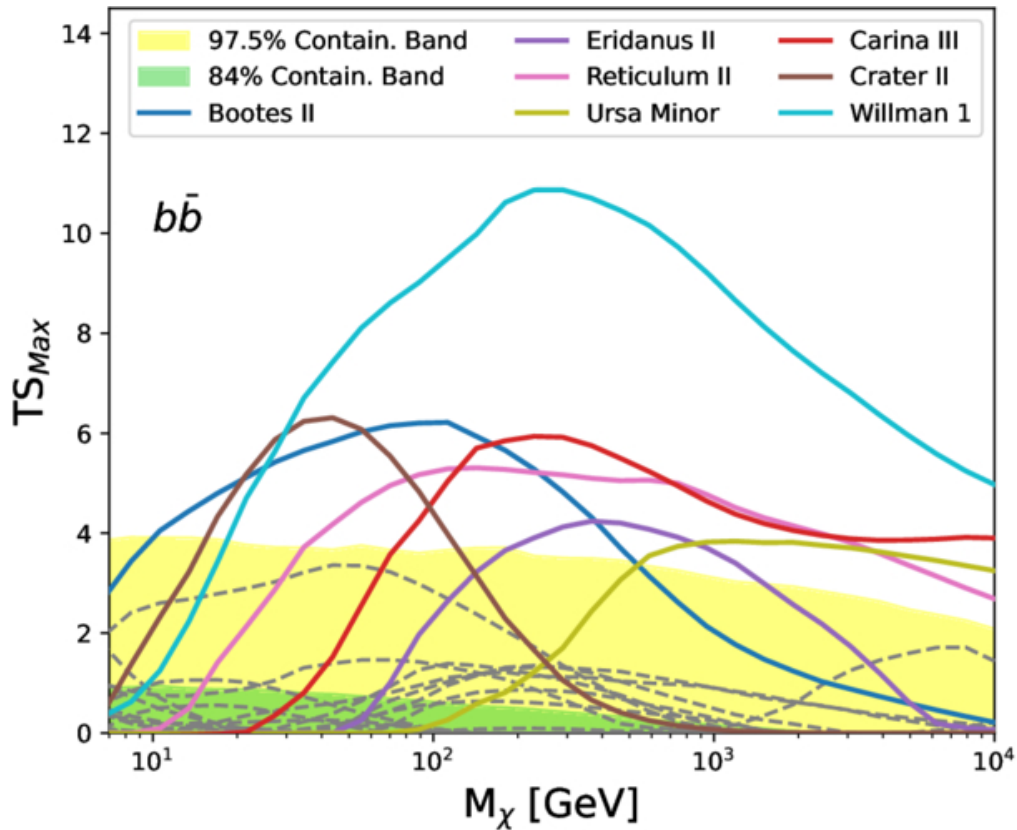
Figure A1. from Antonio Circiello et al 2026 Astrophys. J. Lett. 1004 doi:10.3847/2041-8213/ae71c7 https://dx.doi.org/10.3847/2041-8213/ae71c7 © 2026. The Author(s). Published by the American Astronomical Society.
