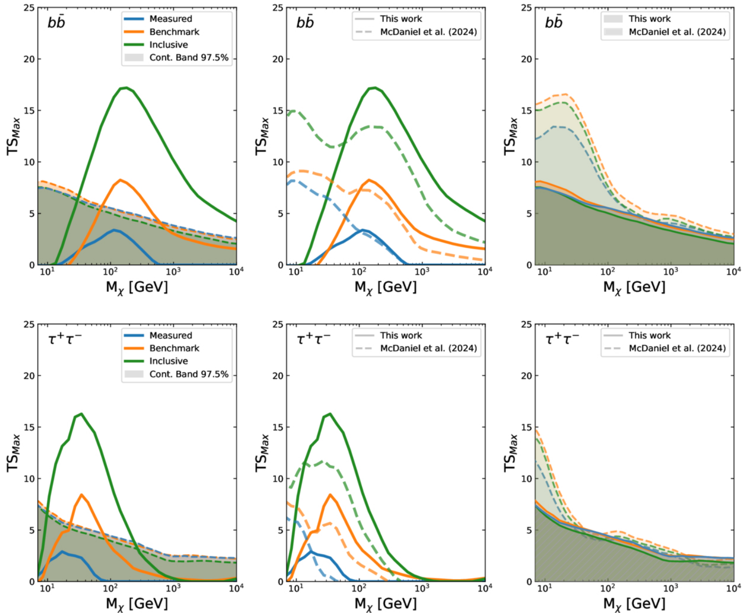
Figure 4. from Antonio Circiello et al 2026 Astrophys. J. Lett. 1004 doi:10.3847/2041-8213/ae71c7 https://dx.doi.org/10.3847/2041-8213/ae71c7 © 2026. The Author(s). Published by the American Astronomical Society.
