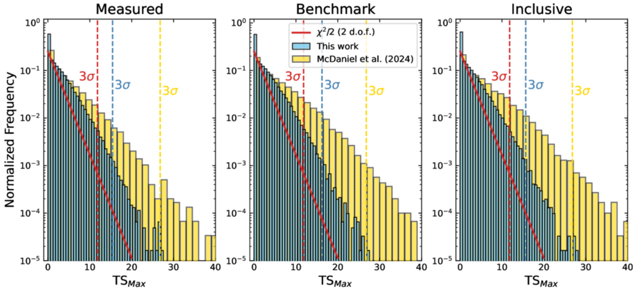
Figure 3. from Antonio Circiello et al 2026 Astrophys. J. Lett. 1004 doi:10.3847/2041-8213/ae71c7 https://dx.doi.org/10.3847/2041-8213/ae71c7 © 2026. The Author(s). Published by the American Astronomical Society.
