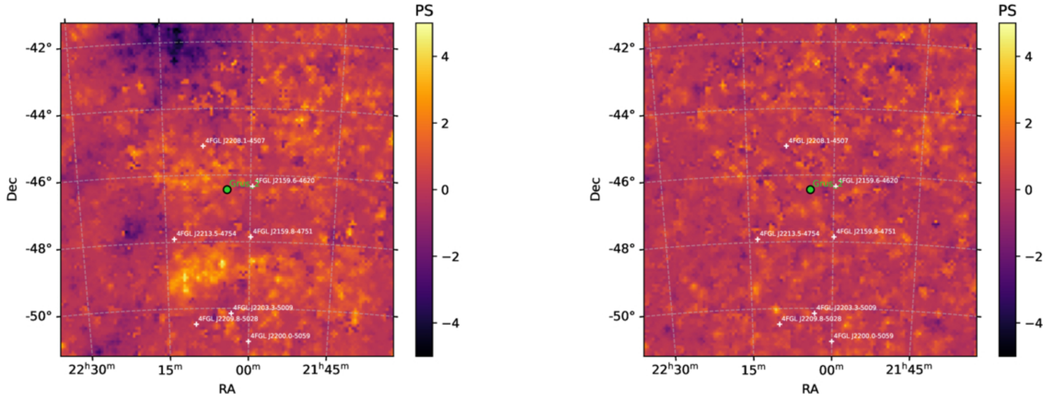
Figure 1. from Antonio Circiello et al 2026 Astrophys. J. Lett. 1004 doi:10.3847/2041-8213/ae71c7 https://dx.doi.org/10.3847/2041-8213/ae71c7 © 2026. The Author(s). Published by the American Astronomical Society.
