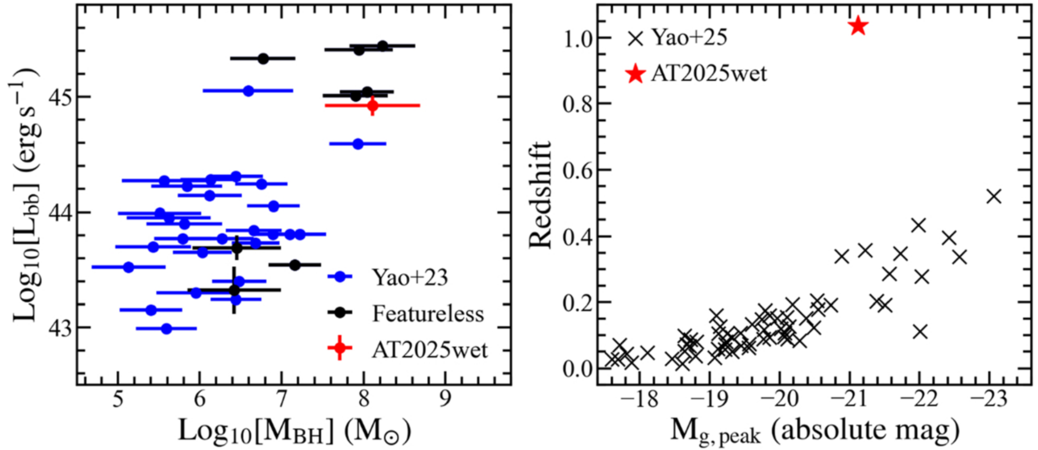
Figure 6. from Jiazheng Zhu et al 2026 Astrophys. J. Lett. 1004 doi:10.3847/2041-8213/ae710d https://dx.doi.org/10.3847/2041-8213/ae710d © 2026. The Author(s). Published by the American Astronomical Society.
