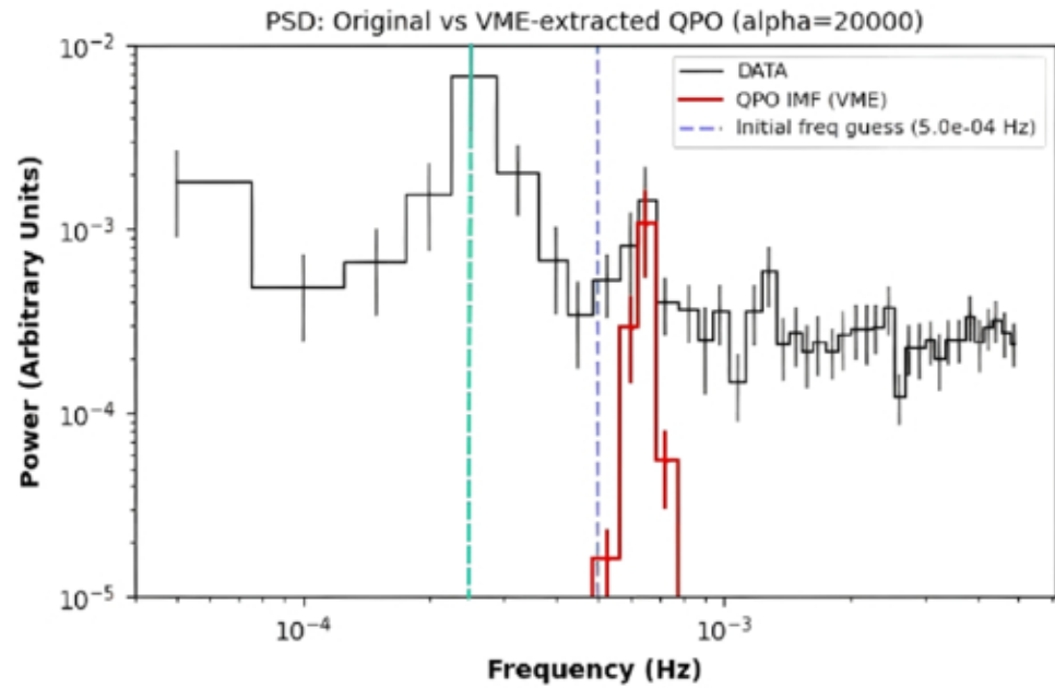
Figure 9. from Wen-Zhong Li et al 2026 Astrophys. J. Lett. 1005 doi:10.3847/2041-8213/ae7106 https://dx.doi.org/10.3847/2041-8213/ae7106 © 2026. The Author(s). Published by the American Astronomical Society.
